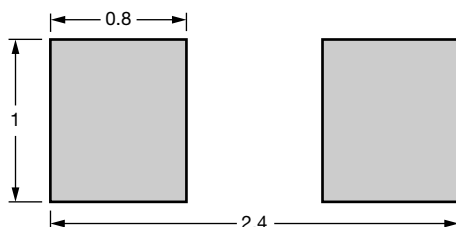
Recommended solder land pattern dimensions (mm)
