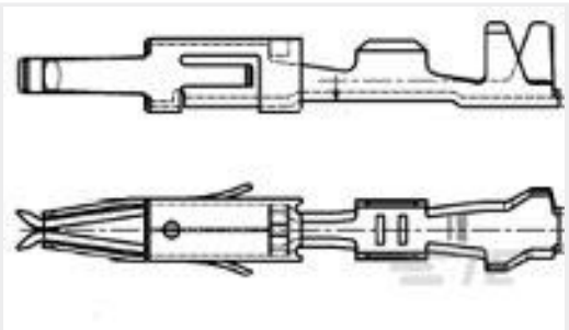
TE Part #9637111-1 MICRO TIM REC-CONTACT
