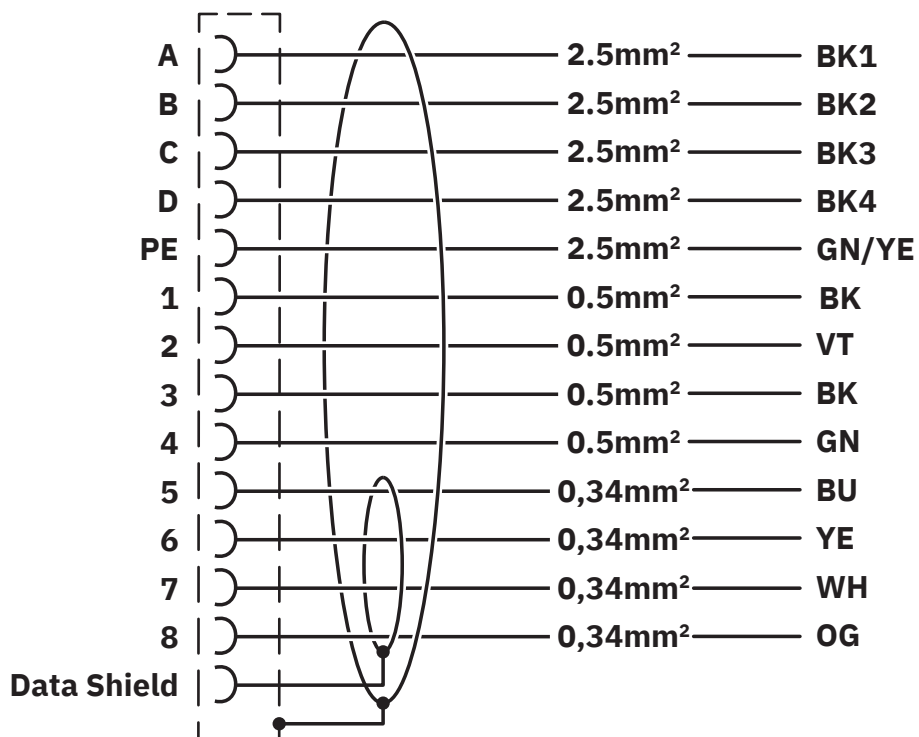
Contact assignment of M23 plugs/sockets
