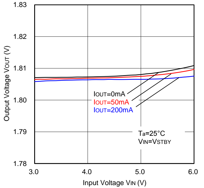
Figure 4. Line Regulation
