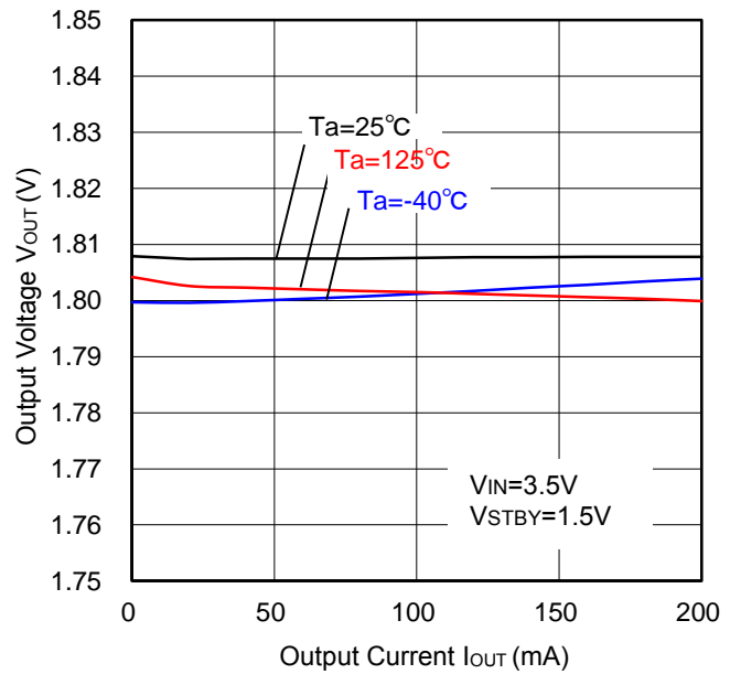
Figure 6. Load Regulation
