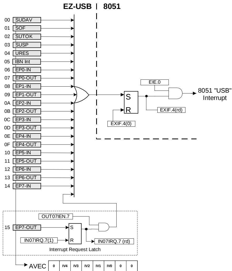
Figure 9-2. USB Interrupts
