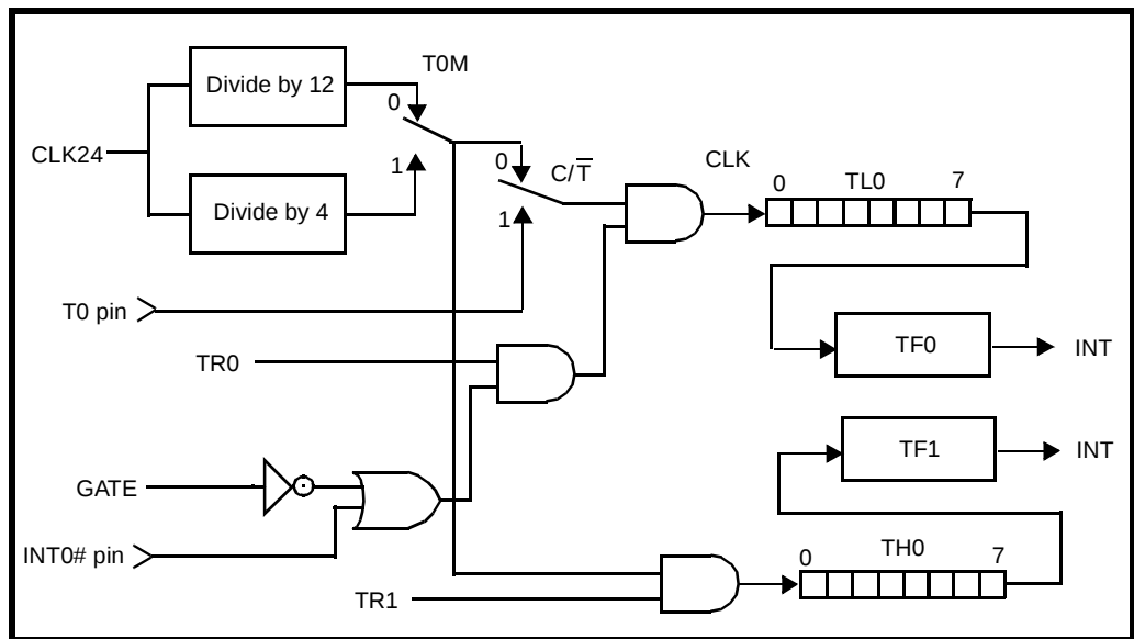
Figure C-3. Timer 0 - Mode 3
