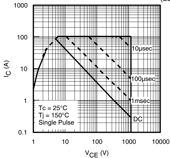
Fig. 2 - Forward SOA
