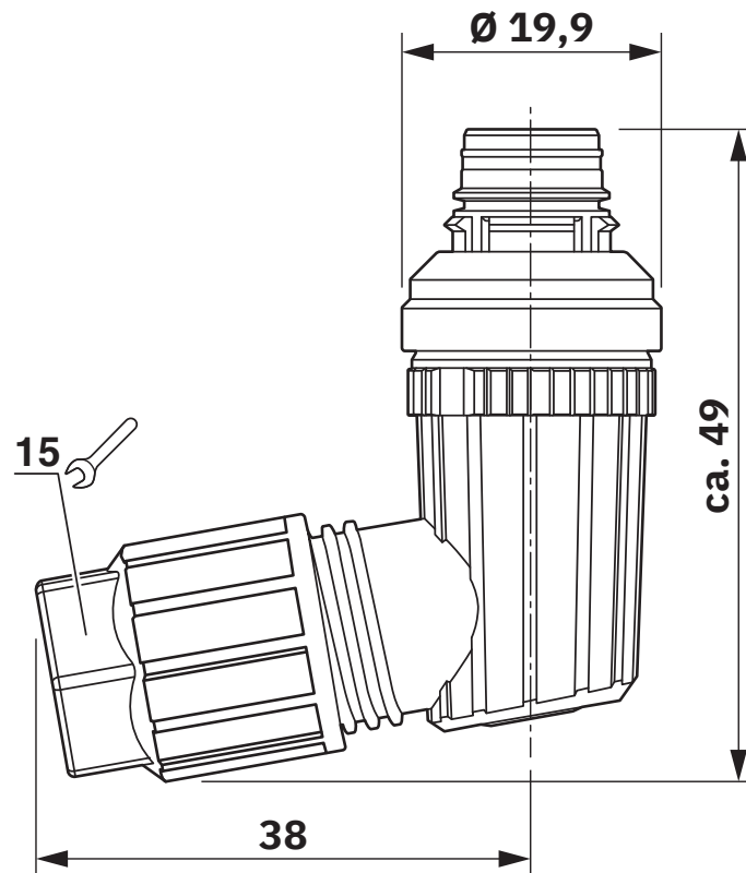
Dimensional drawing
