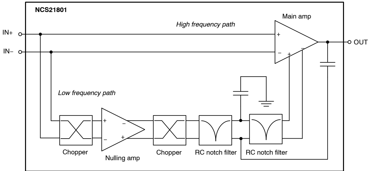
Figure 39. Simplified Schematic of the Chopper-stabilized Amplifier Architecture
