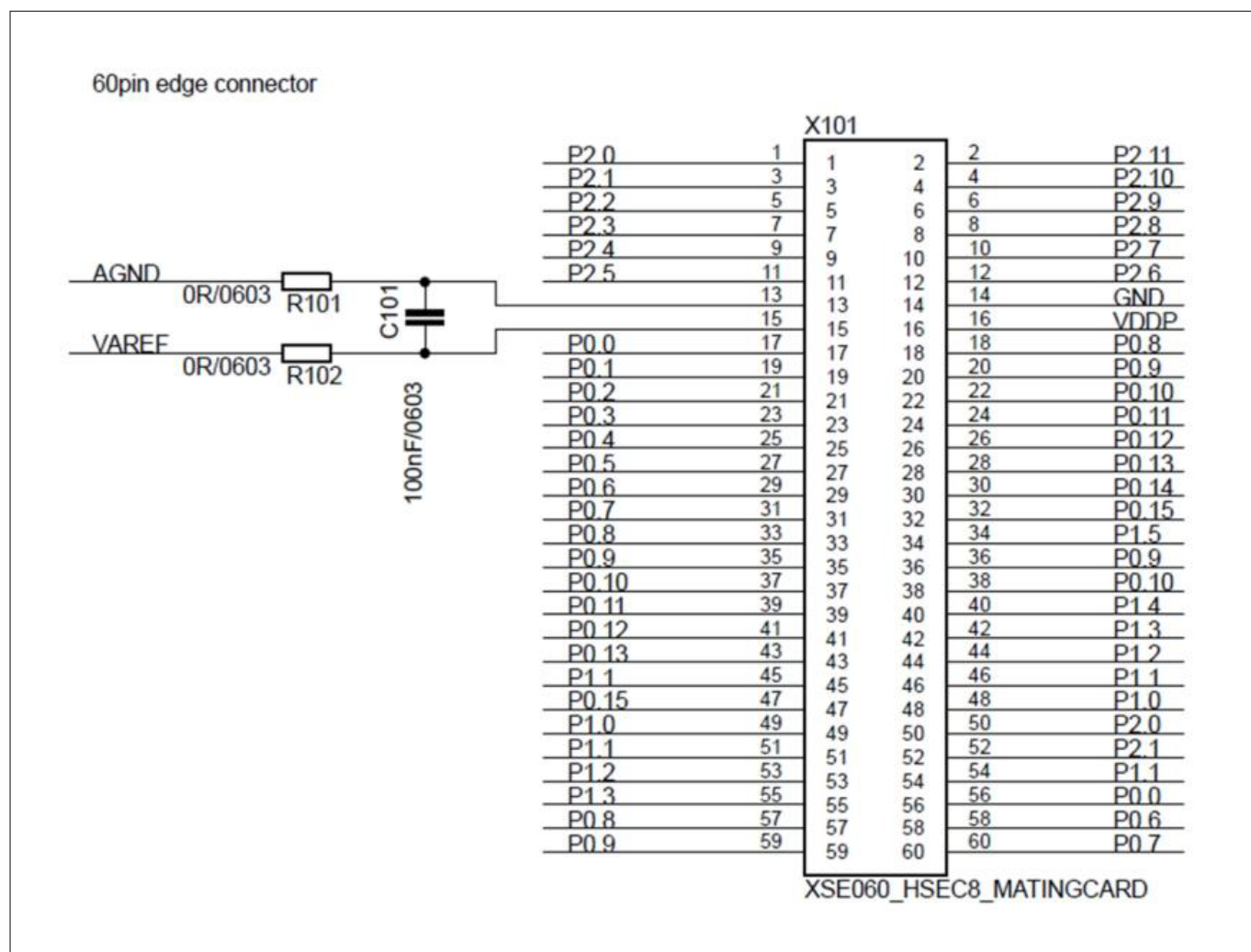
Figure 6 Pinout of the 2x30 pin edge connector
