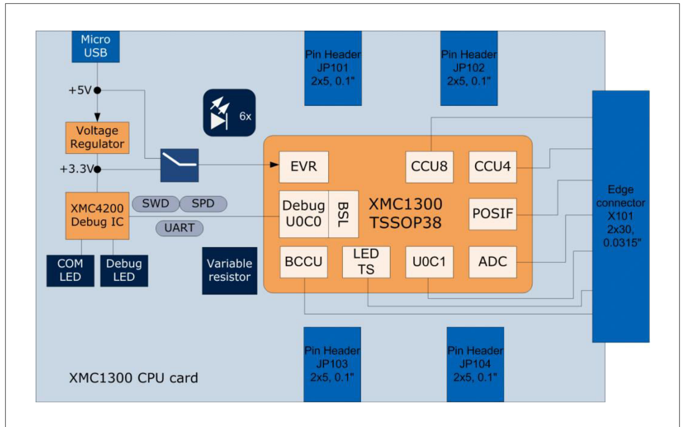
Figure 1 Block Diagram of XMC1300 CPU Card
