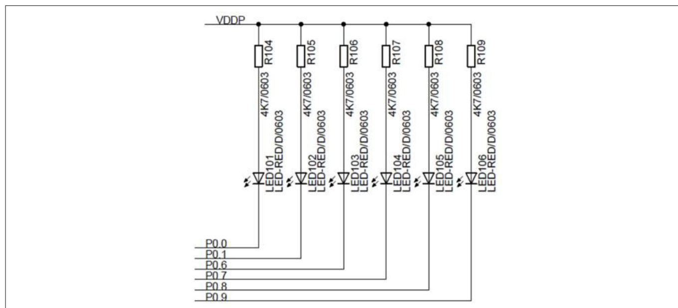
Figure 4 LEDs circuit
