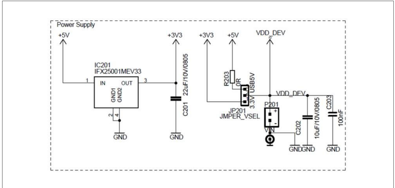
Figure 3 Power Supply circuit
