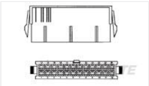
TE Part #2-1586861-4 24P PM PLUG VAL-U-LOK PM GW
