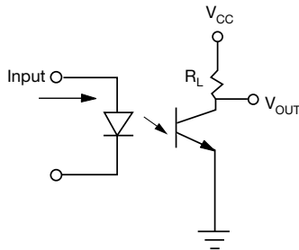
Fig. 1 - Test Circuit
