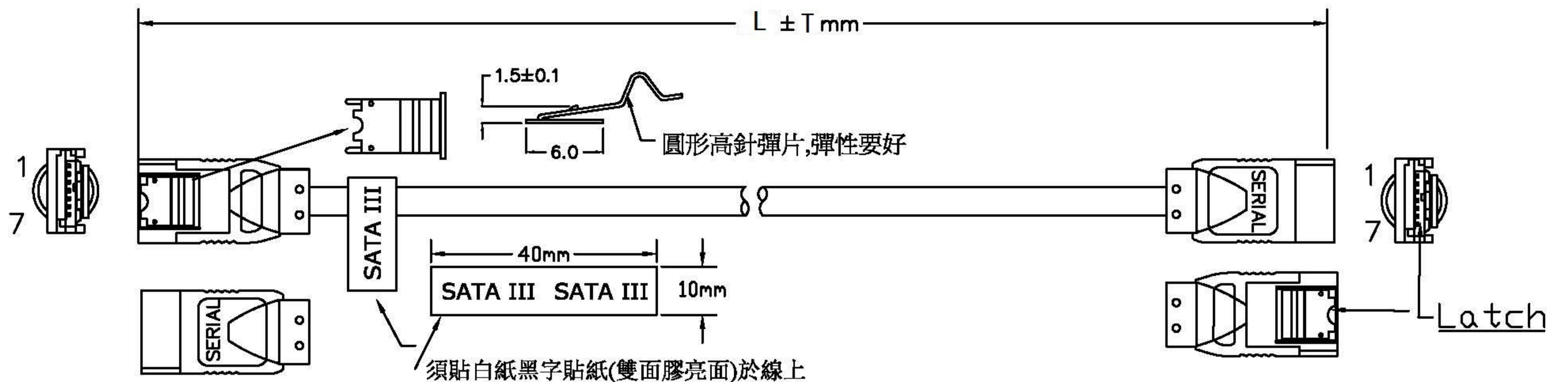
SERIAL ATA 7P (WITH Latch)
