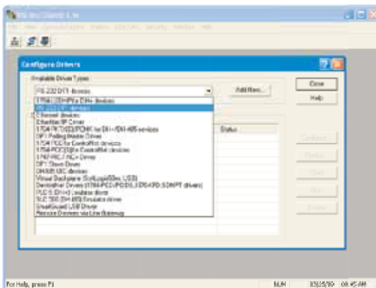
Figure 4.3.21d Configurer pilotes.
