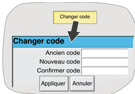
Figure 4.4.5 Changer code
