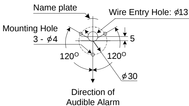
Mounting Dimensions
