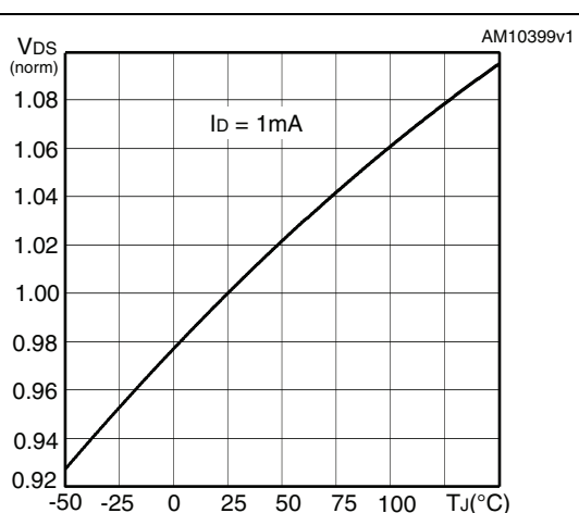
Figure 13. Normalized V_{DSS} vs temperature
