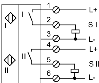
[C2] Screw terminal
