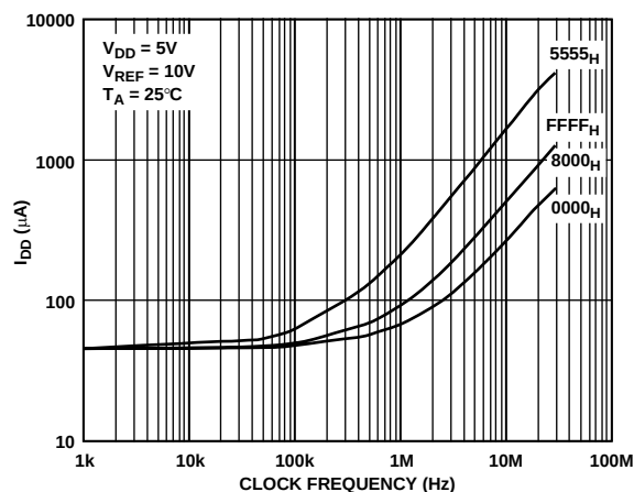
Figure 20. AD5554 Power Supply Current vs. Clock Frequency
