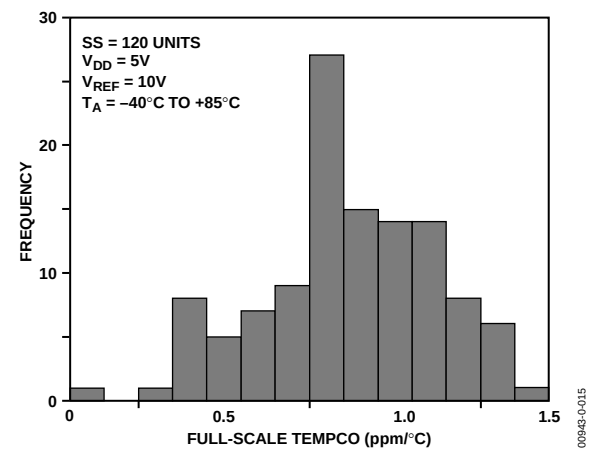
Figure 15. AD5544 Full-Scale Tempco (ppm/°C)
