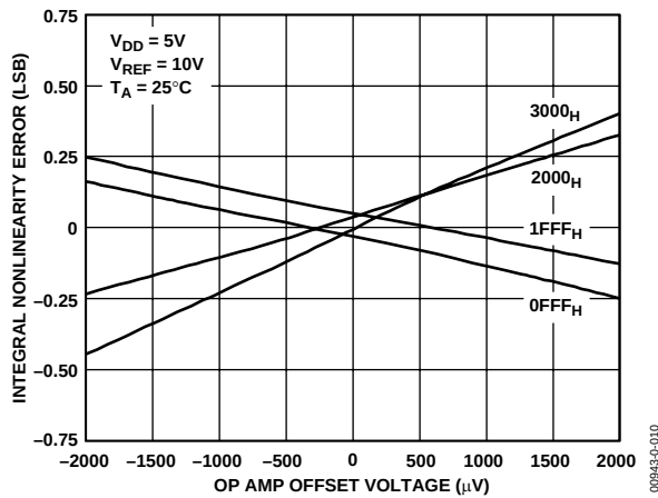
Figure 10. AD5554 Integral Nonlinearity Error vs. Op Amp Offset
