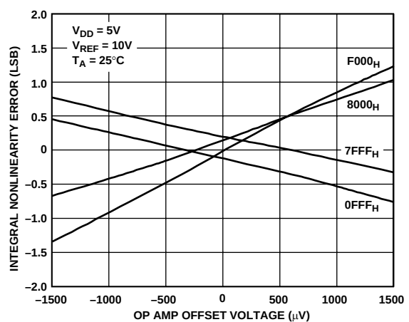
Figure 9. AD5554 Integral Nonlinearity Error vs. Op Amp Offset
