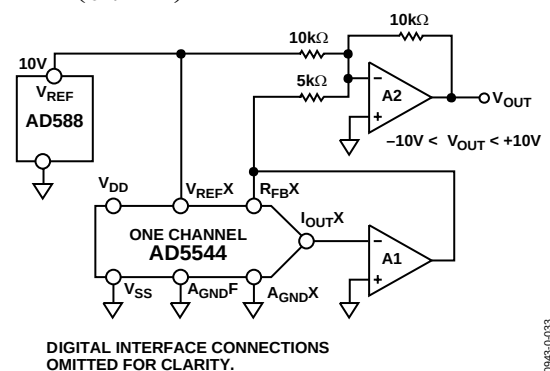
Figure 33. Four-Quadrant Multiplying Application Circuit
