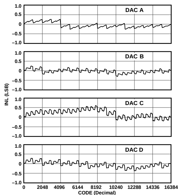
Figure 7. AD5554 INL vs. Code, T_A = 25^\circ\text{C}
