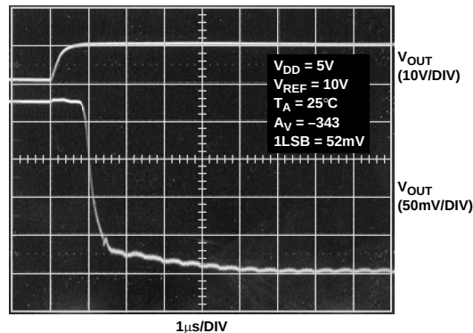
Figure 19. AD5554 Small Signal Settling Time
