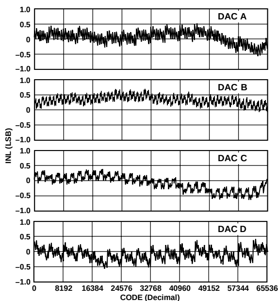
Figure 2. AD5544 INL vs. Code Plot ( T_A = 25^\circ\text{C} )
