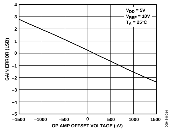
Figure 14. AD5554 Gain Error vs. Op Amp Offset
