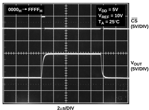
Figure 18. AD5554 Large Signal Settling Time
