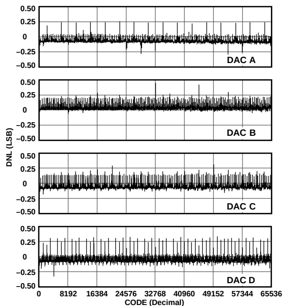
Figure 6. AD5554 DNL vs. Code, T_A = 25^\circ\text{C}
