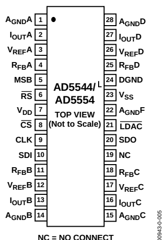
Figure 3. AD5544/AD5554 Pin Configuration
