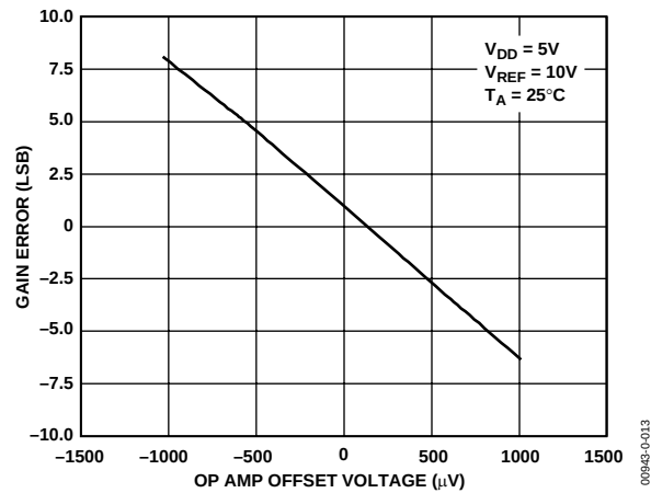
Figure 13. AD5544 Gain Error vs. Op Amp Offset
