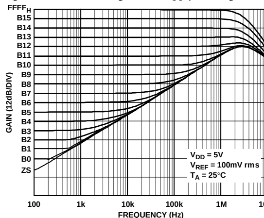
Figure 26. AD5554 Reference Multiplying Bandwidth vs. Code
