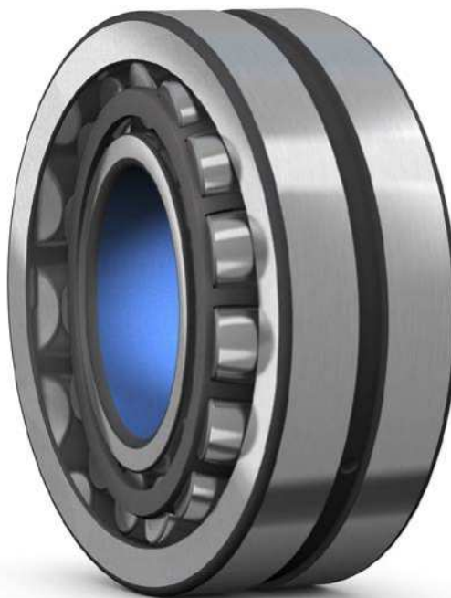
SKF spherical roller bearing with a PTFE-coated bore
