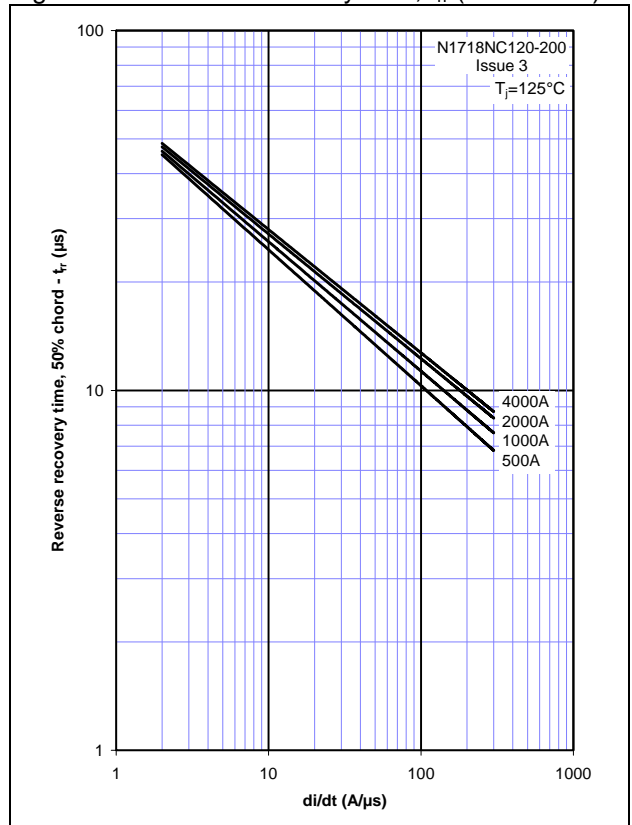
Figure 8 - Maximum recovery time, t_r (50% chord)
