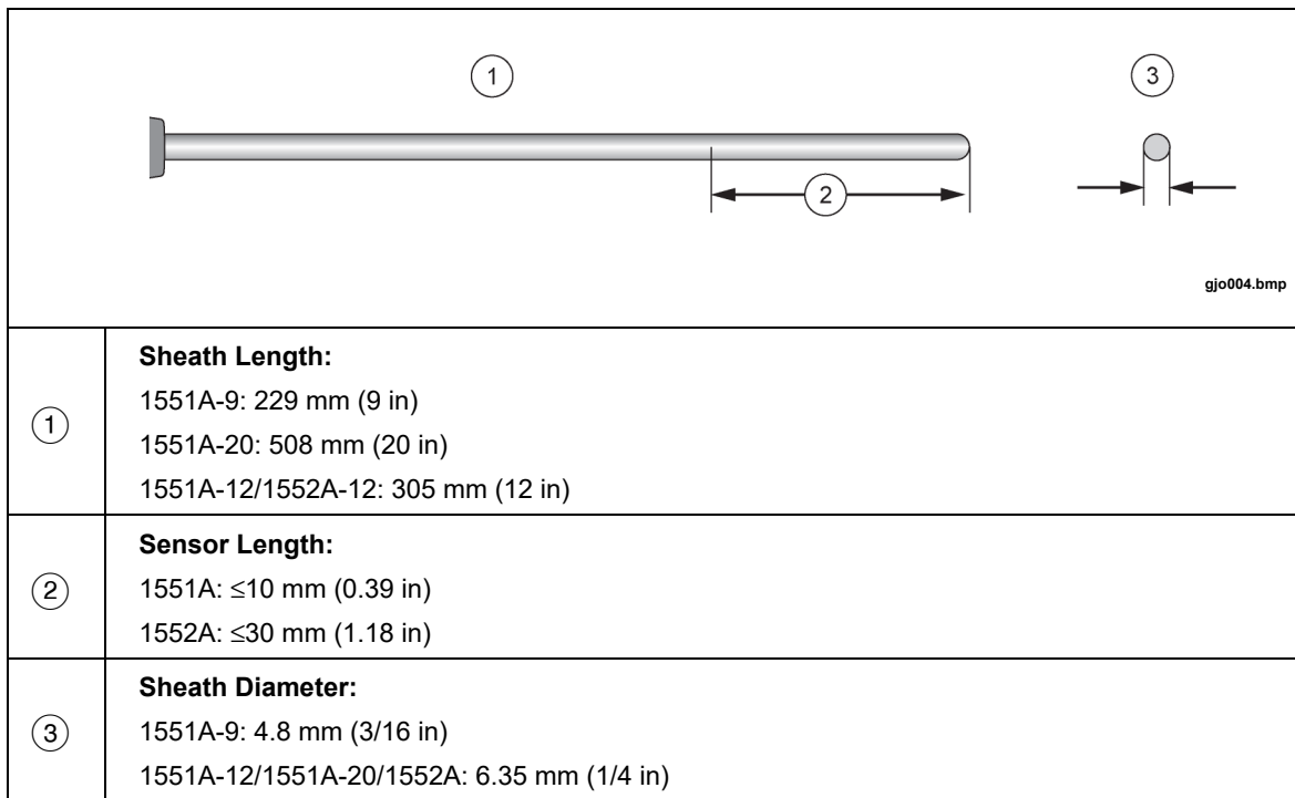
Figure 1. Probe Measurements
