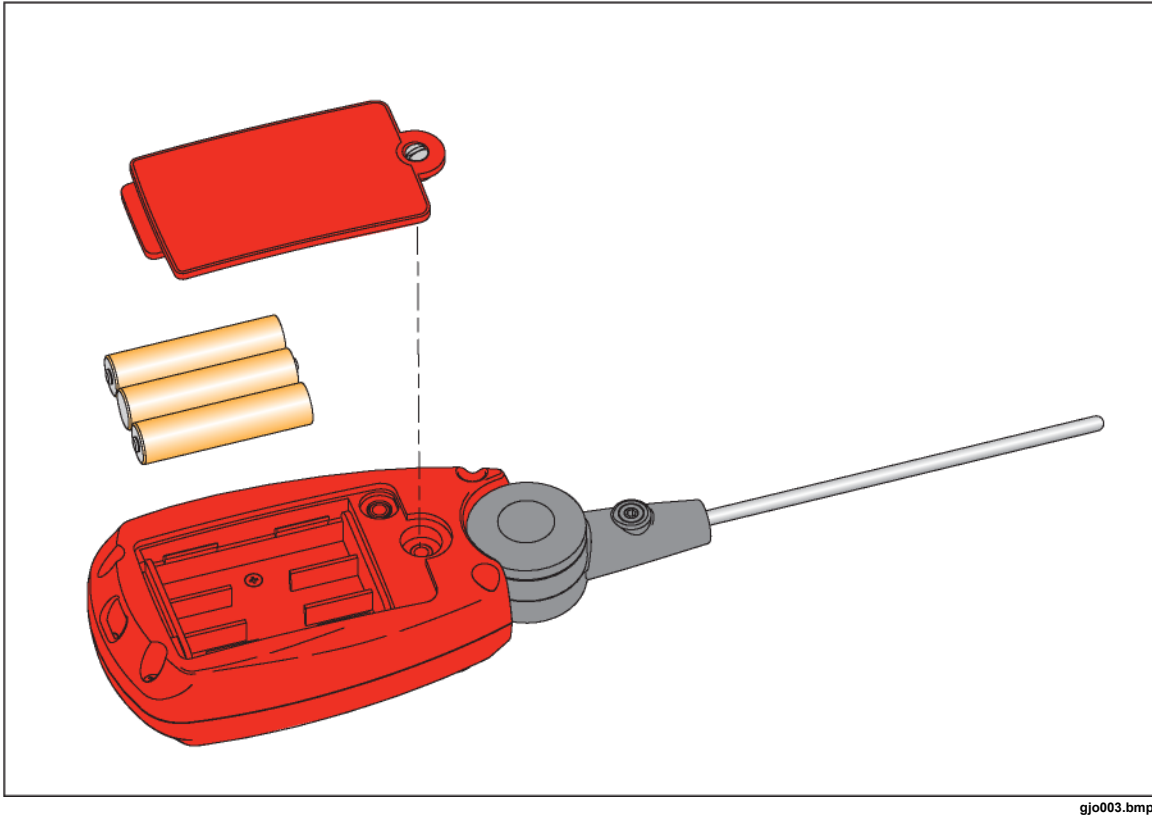
Figure 4. Battery Replacement
