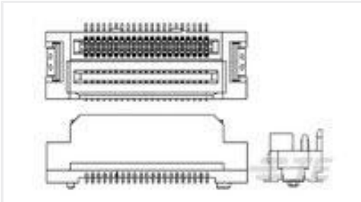
TE Part #2069389-1 Z-STACK CONN. 42P ASS'Y F8
