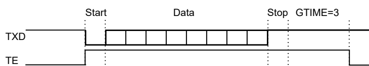
Figure 34-16. Example of TE Drive with Guard Time
