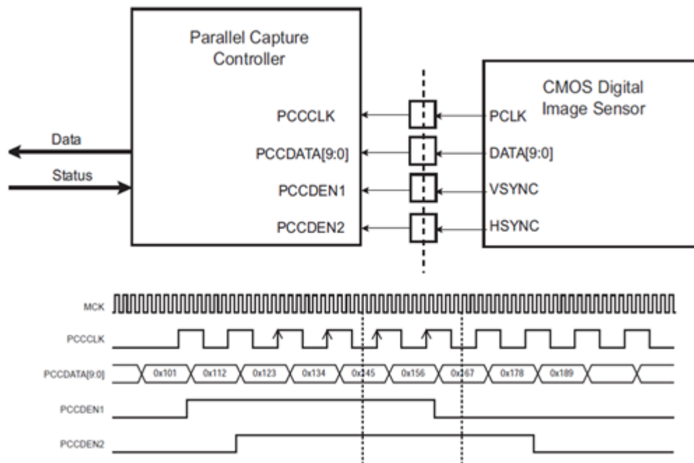
Figure 54-21. PCC Signaling
