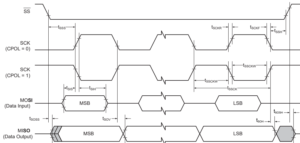
Figure 54-8. SPI Timing Requirements in Client Mode
