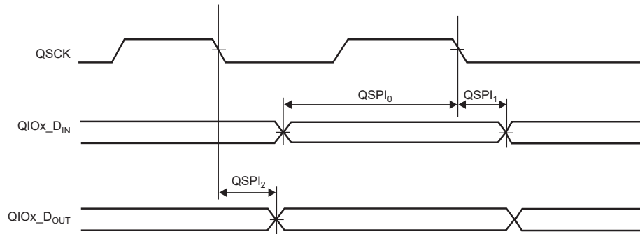
Figure 54-10. QSPI SDR Host Mode 1
