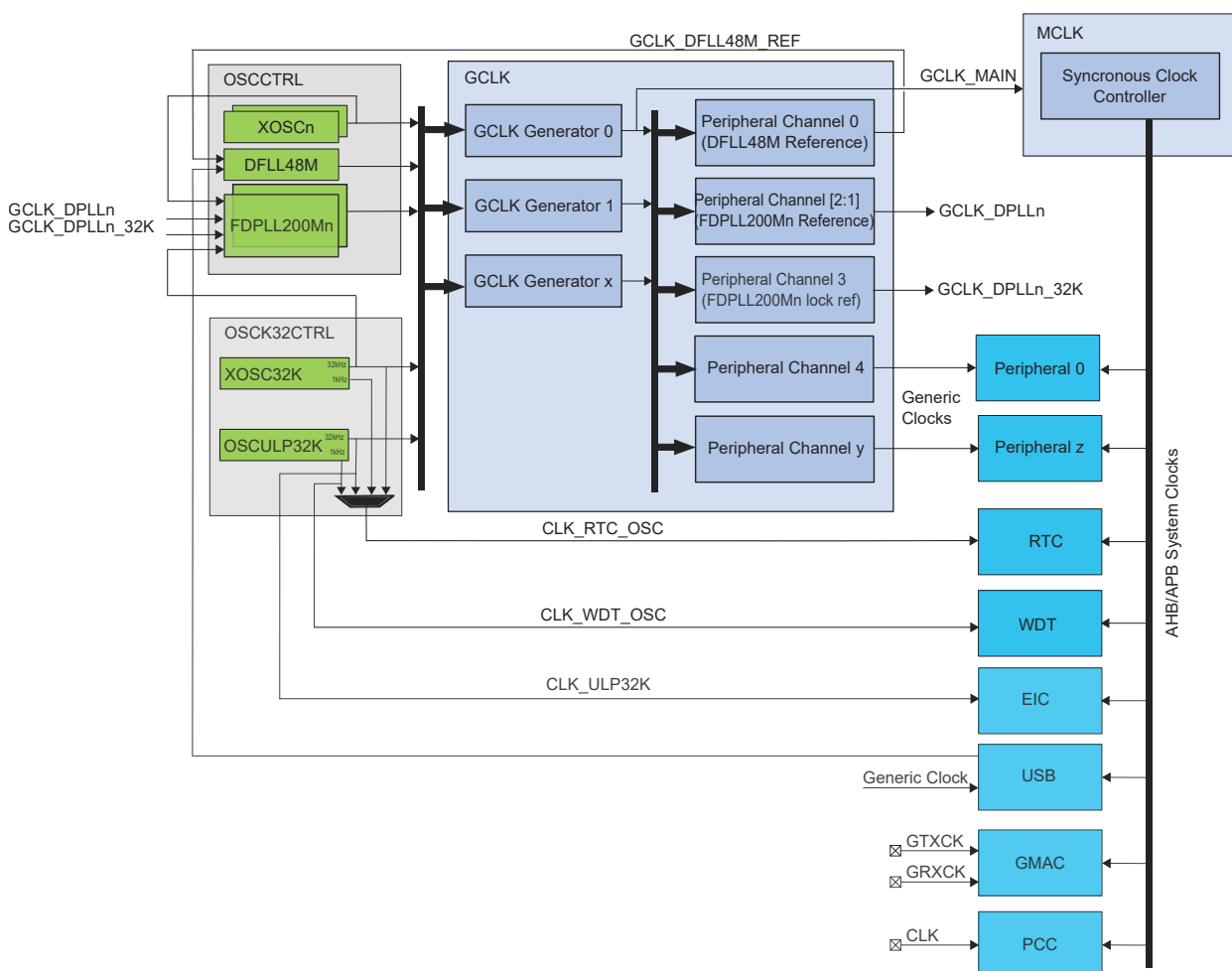
Figure 13-1. Clock Distribution
