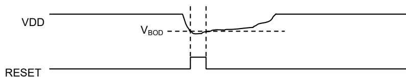
Figure 55-2. BOD33 Hysteresis OFF
