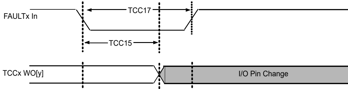
Figure 54-27. TCCx Timer Compare Fault Output Module Timing Diagrams
