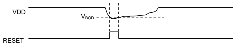
Figure 56-2. BOD33 Hysteresis OFF
