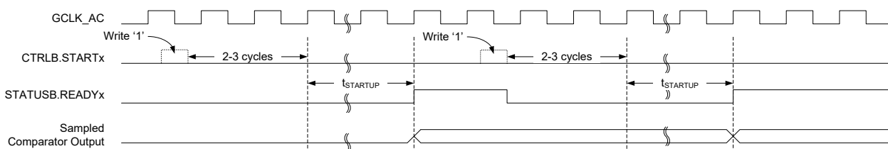
Figure 46-3. Single-Shot Example
