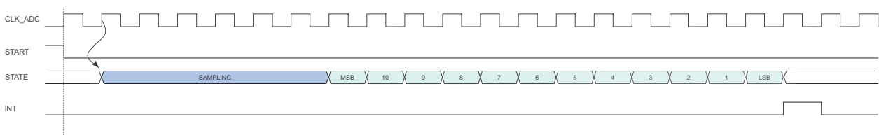
Figure 45-4. ADC Timing for One Conversion with Increased Sampling Time, 12-bit
