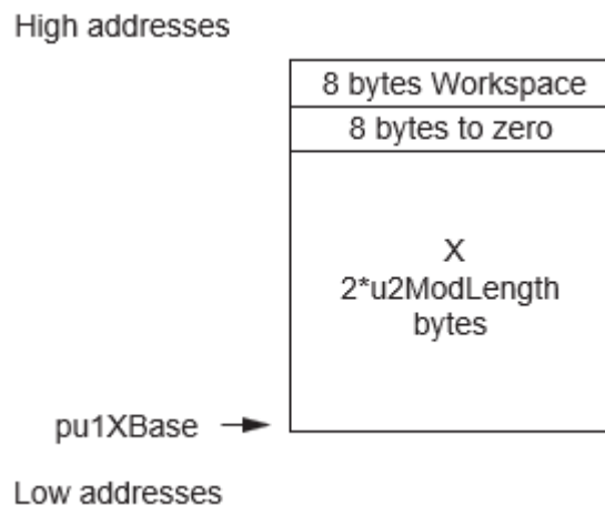
Figure 43-3. Value X in \{\text{nu1XBase}, 2 * \text{u2ModLength} + 16\}
