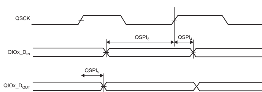
Figure 54-10. QSPI SDR Host Mode 1
