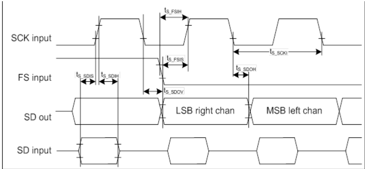
Figure 54-19. Client Mode: SCK and FS are Input
