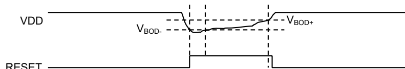
Figure 54-3. BOD33 Hysteresis ON
