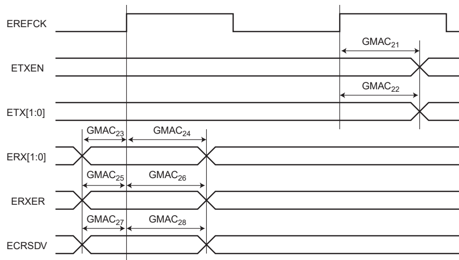
Figure 54-17. GMAC RMII Mode Signals
