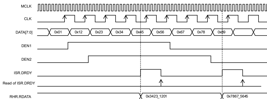
Figure 52-6. PCC Waveforms (DSIZE=4_DATA, ALWAYS = 1, HALFS = 0)
