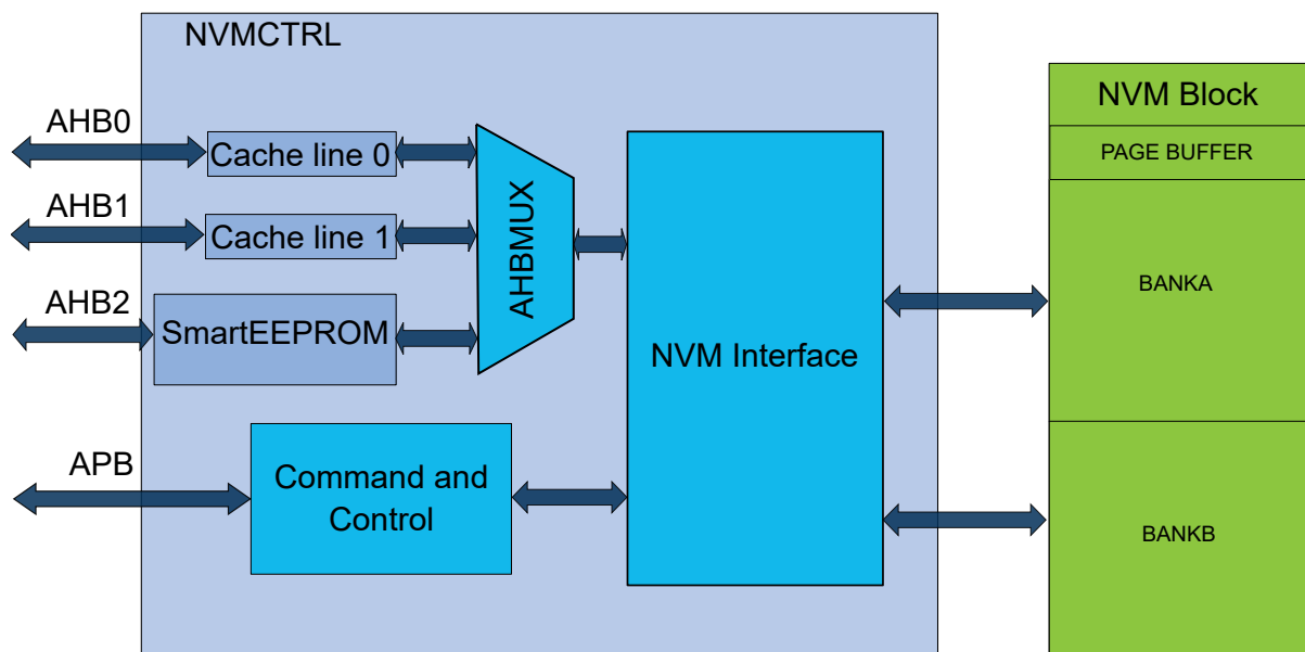
Figure 25-1. Block Diagram
