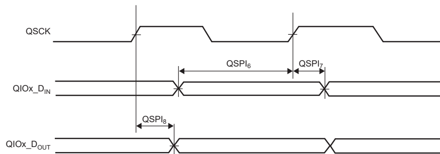
Figure 54-11. QSPI SDR Host Mode 2
