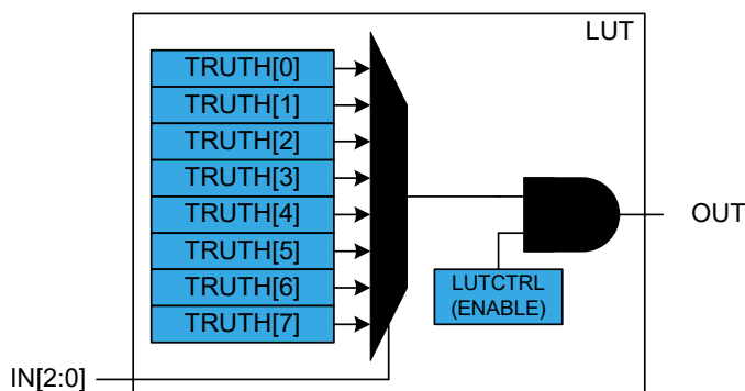
Figure 41-2. Truth Table Output Value Selection
