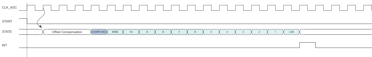
Figure 45-5. ADC Timing for One Conversion with Offset Compensation, 12-bit
