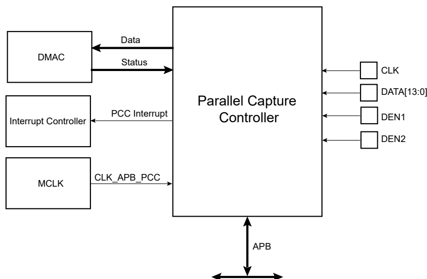
Figure 52-1. Block Diagram
