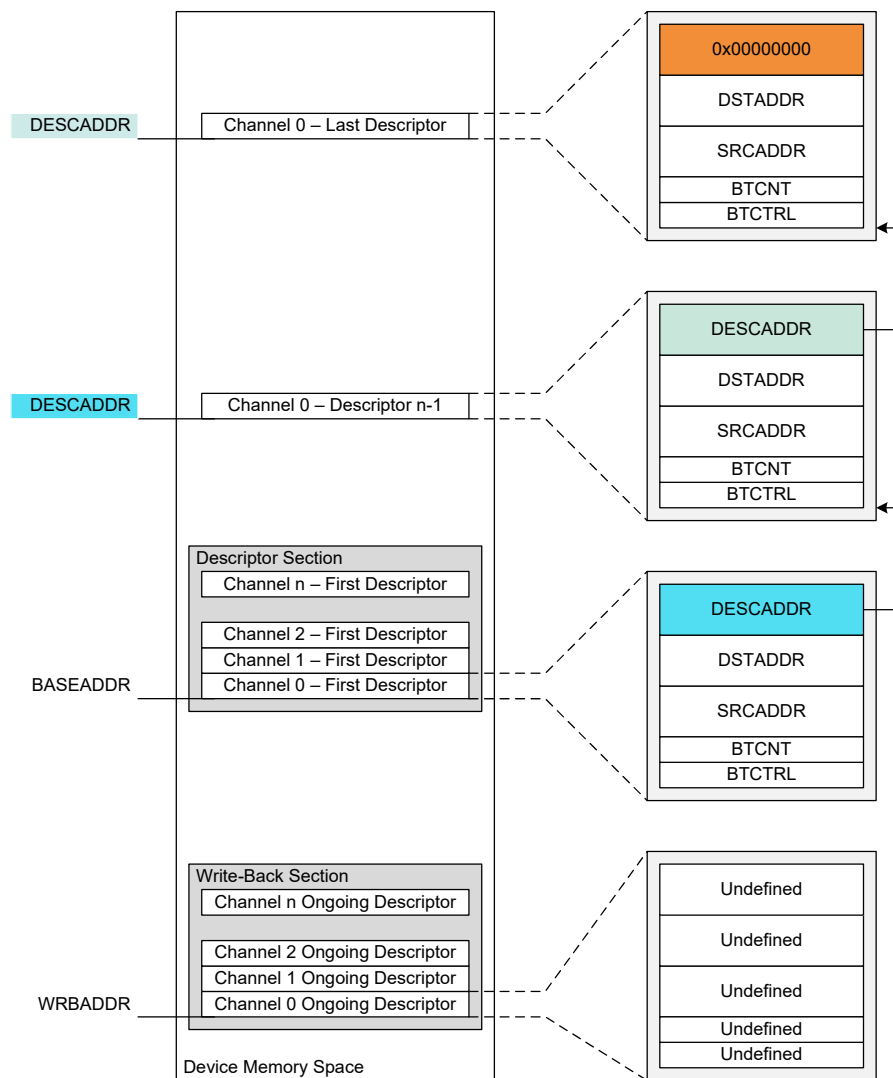
Figure 22-3. Memory Sections
