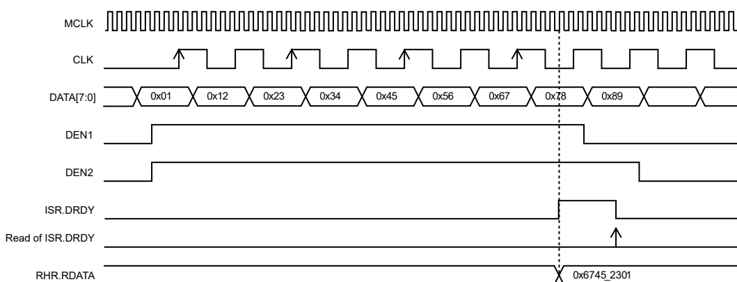
Figure 52-9. PCC Waveforms (DSIZE=4_DATA, ALWAYS = 0, HALFS = 1, FRSTS = 0)
