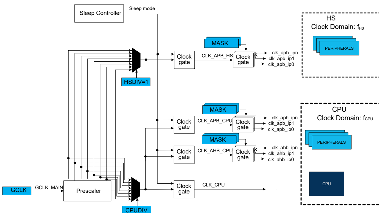
Figure 15-2. Synchronous Clock Selection and Prescaler
