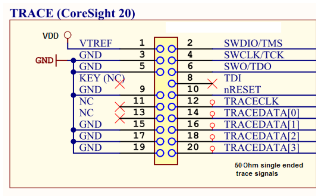
Figure 60-16. Trace (CoreSight 20) Connector Diagram
