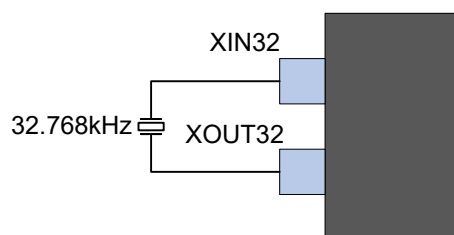
Figure 60-10. External Real Time Oscillator without Load Capacitor
