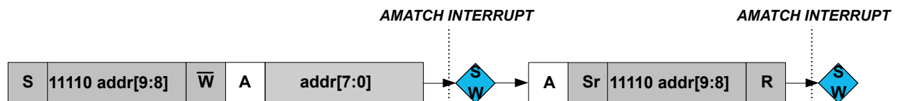
Figure 36-11. 10-bit Addressing
