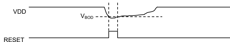
Figure 19-2. BOD Hysteresis Principle
