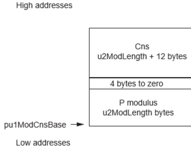
Figure 43-7. Modulus P and Cns{pu1ModCnsBase, 2 * u2ModLength + 16 }
