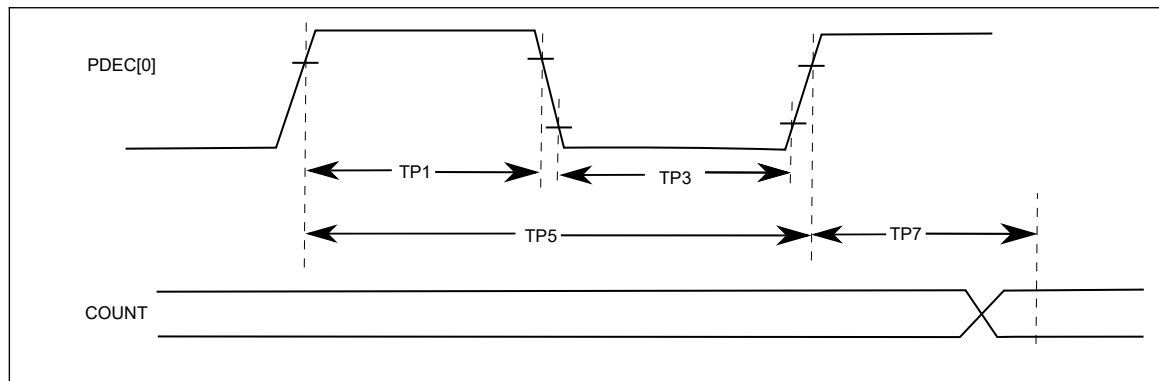
Figure 54-28. Position Decoder (PDEC) Timing Diagrams Counter Mode
