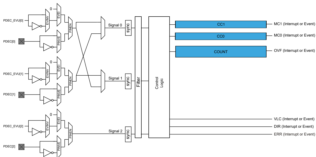
Figure 53-1. Block Diagram
