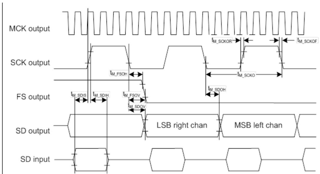
Figure 54-18. Host Mode: SCK, FX, and MCK are Output
