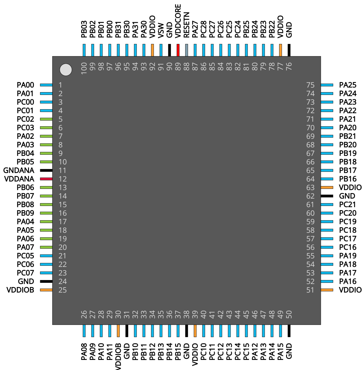
Figure 4-3. 100-Pin TQFP Package
