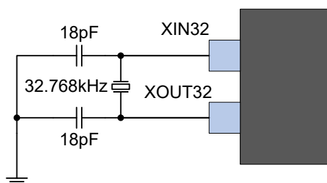
Figure 60-11. External Real Time Oscillator with Load Capacitor
