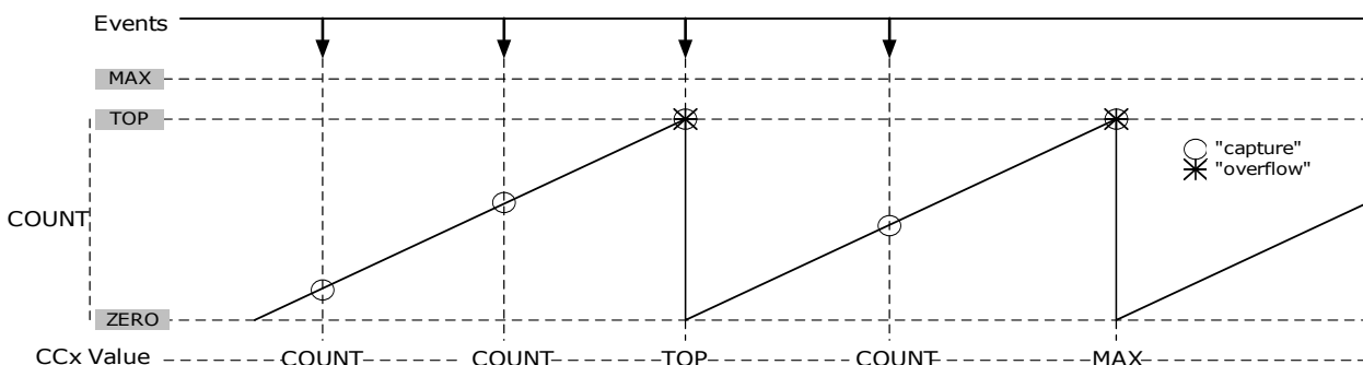
Figure 48-15. Time Stamp
