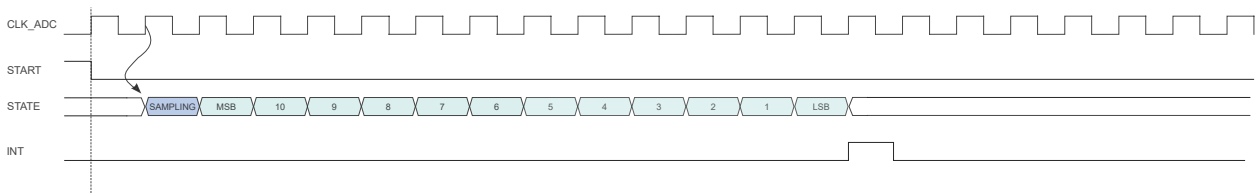
Figure 45-3. ADC Timing for One Conversion in 12-bit Resolution
