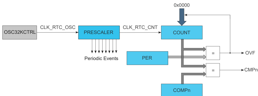
Figure 21-2. RTC Block Diagram (Mode 1 — 16-Bit Counter)
