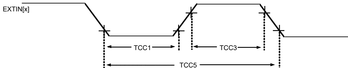
Figure 54-26. TCCx Timer Compare Output Module Timing Diagrams
