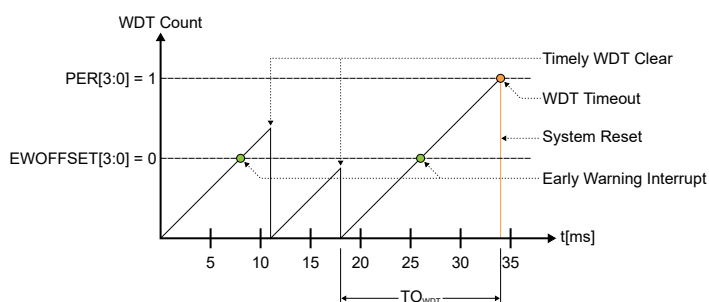
Figure 20-2. Normal-Mode Operation
