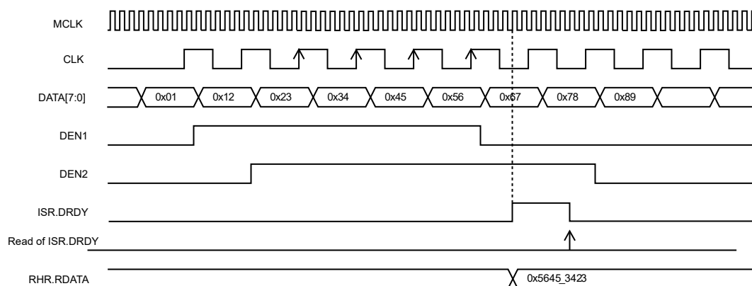
Figure 52-3. PCC Waveforms (DSIZE=4_DATA, ALWYS = 0, HALFS = 0)
