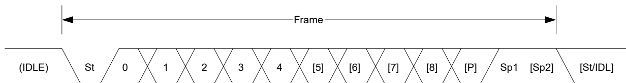
Figure 34-2. Frame Formats
