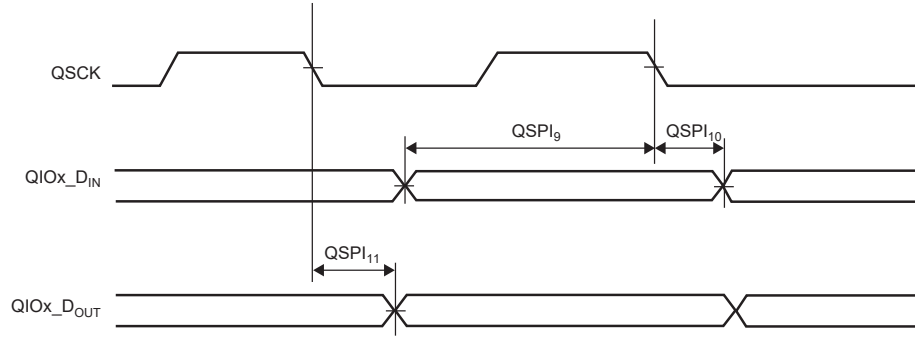
Figure 54-13. QSPI DDR Mode 0 READ
