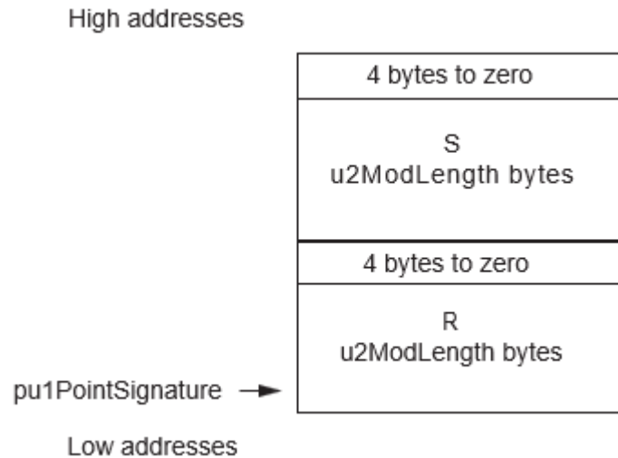
Figure 43-13. PointSignature {pu1PointSignature, 2 * u2ScalarLength + 8}
