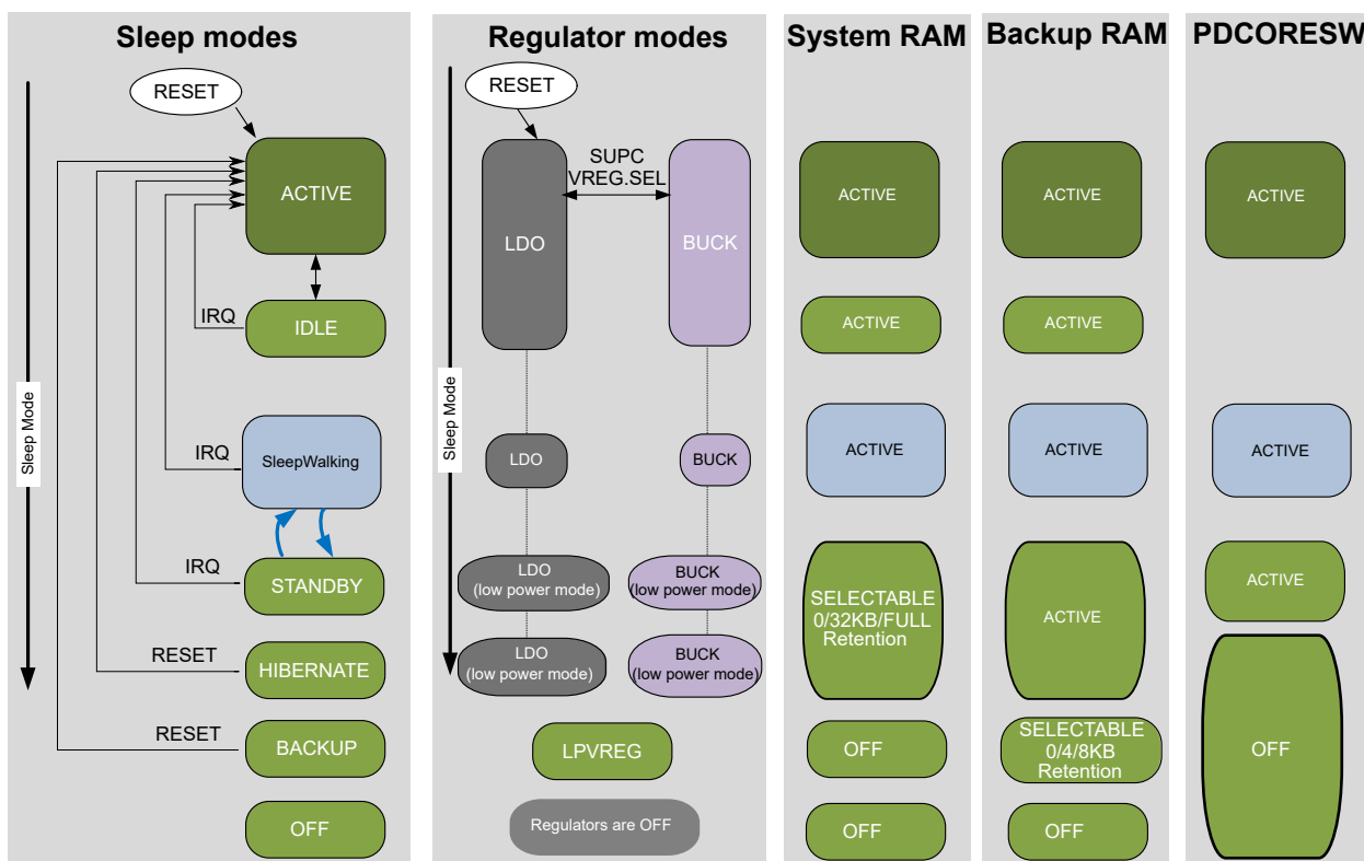
Figure 18-2. Operating Conditions and SleepWalking
