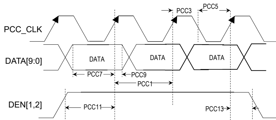
Figure 54-22. PCC - Peripheral Capture Controller Timing Diagrams
