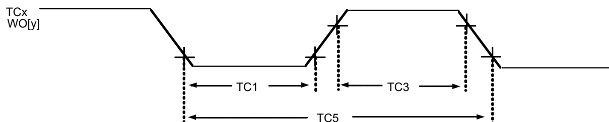
Figure 54-24. TCx Timer Compare Output Module Timing Diagrams
