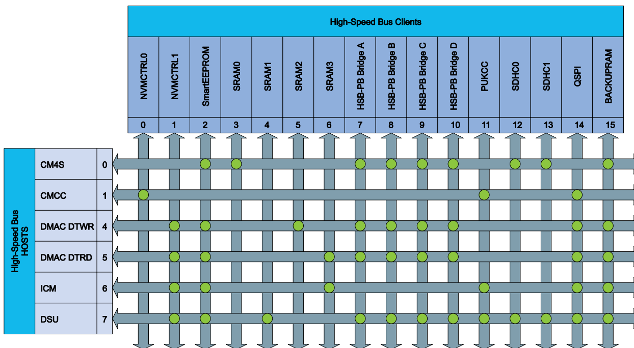
Figure 10-1. Host-Client Relations High-Speed Bus Matrix
