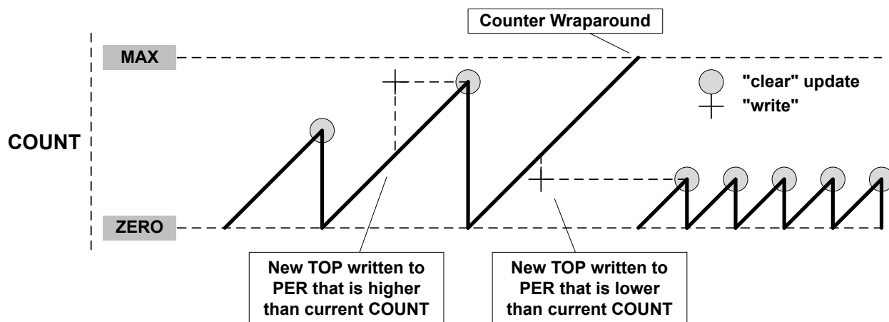
Figure 48-8. Unbuffered Single-Slope Up-Counting Operation
