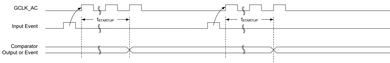
Figure 46-10. Single-Shot SleepWalking
