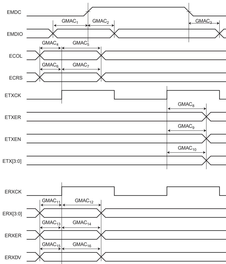
Figure 54-16. GMAC MII Mode Signals
