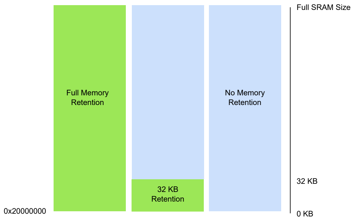
Figure 9-1. Retention Options
