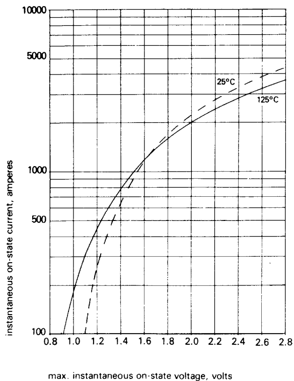
Figure 9 Limit on-state characteristic
