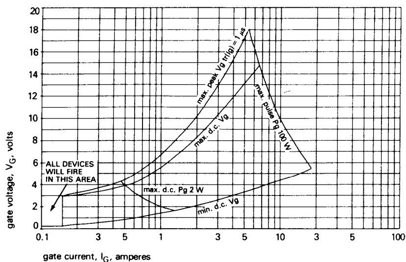
Figure 7 Gate characteristics at 25°C junction temperature
