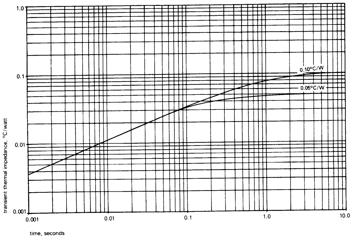
Figure 3 Junction to heatsink thermal impedance
