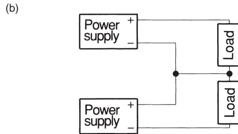
Fig.4.1 Series operation
