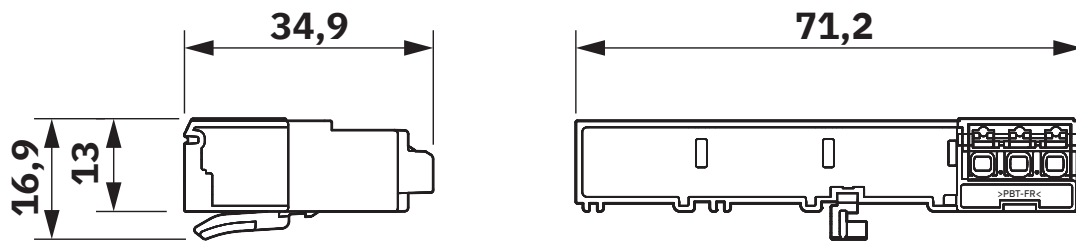
Dimensional drawing
