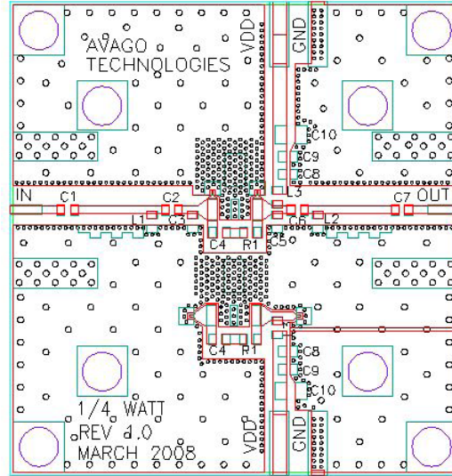
Figure 44. Demoboard
