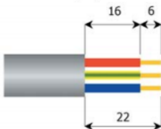
Cable preparation
