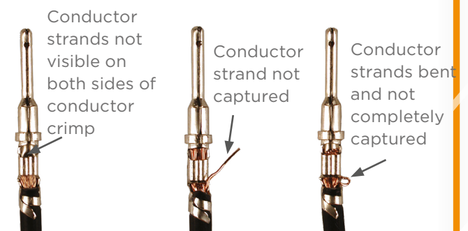
Unacceptable Crimps
