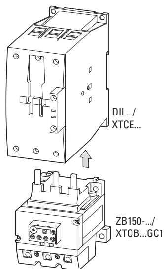
Figure 11: Mounting the ZB150-.../XTOB...GC1
