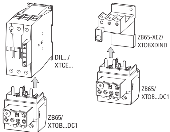
Figure 10: Mounting the ZB65-.../XTOB...DC1
