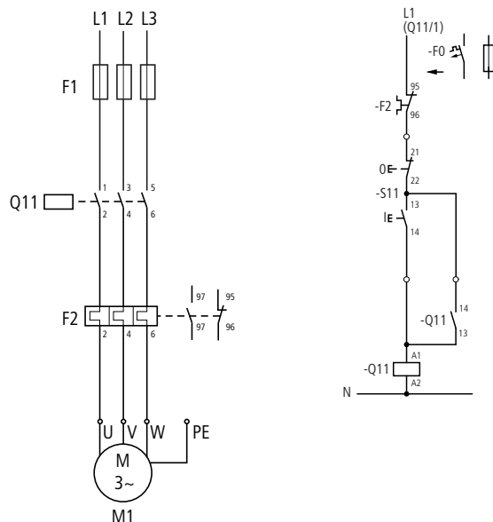
Figure 8: Circuit prevents automatic restart
