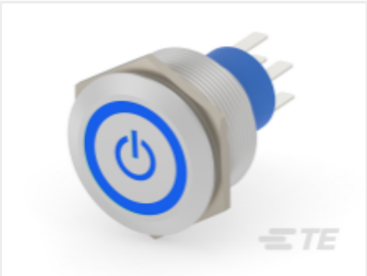
TE Part #2-2317658-5 AV25 DPM 3A MOVING RING POWER BLUE 24V
