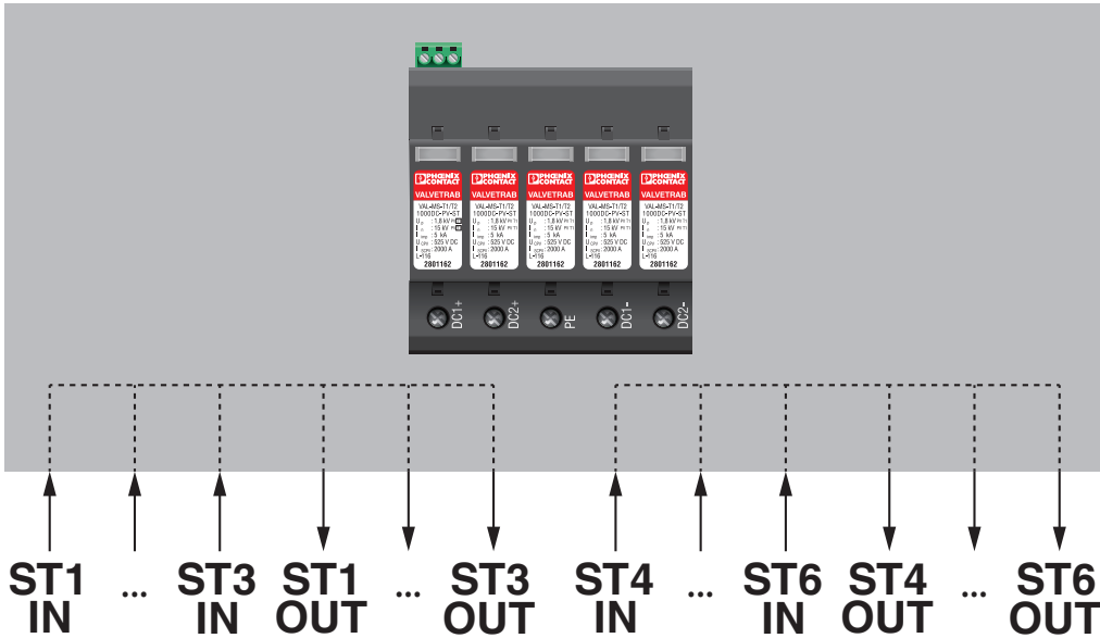
Schematic application drawing
