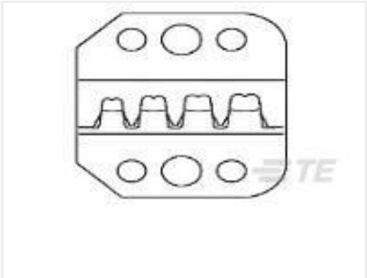
TE Part #58583-2 PROCrimp Die Superseal 1.5 Ser
