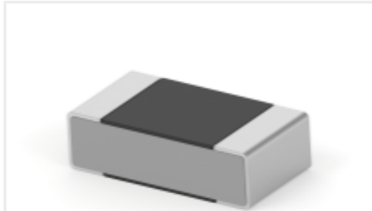
TE Part #1879207-7 RN 0603 232K 0.1% 10PPM 5K RL
