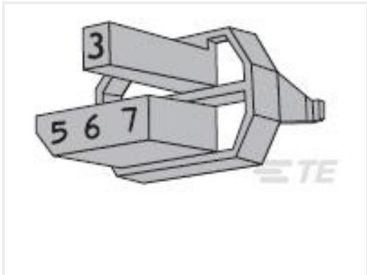
TE Part #6-100526-1 Z-PACK F.CODING KEY
