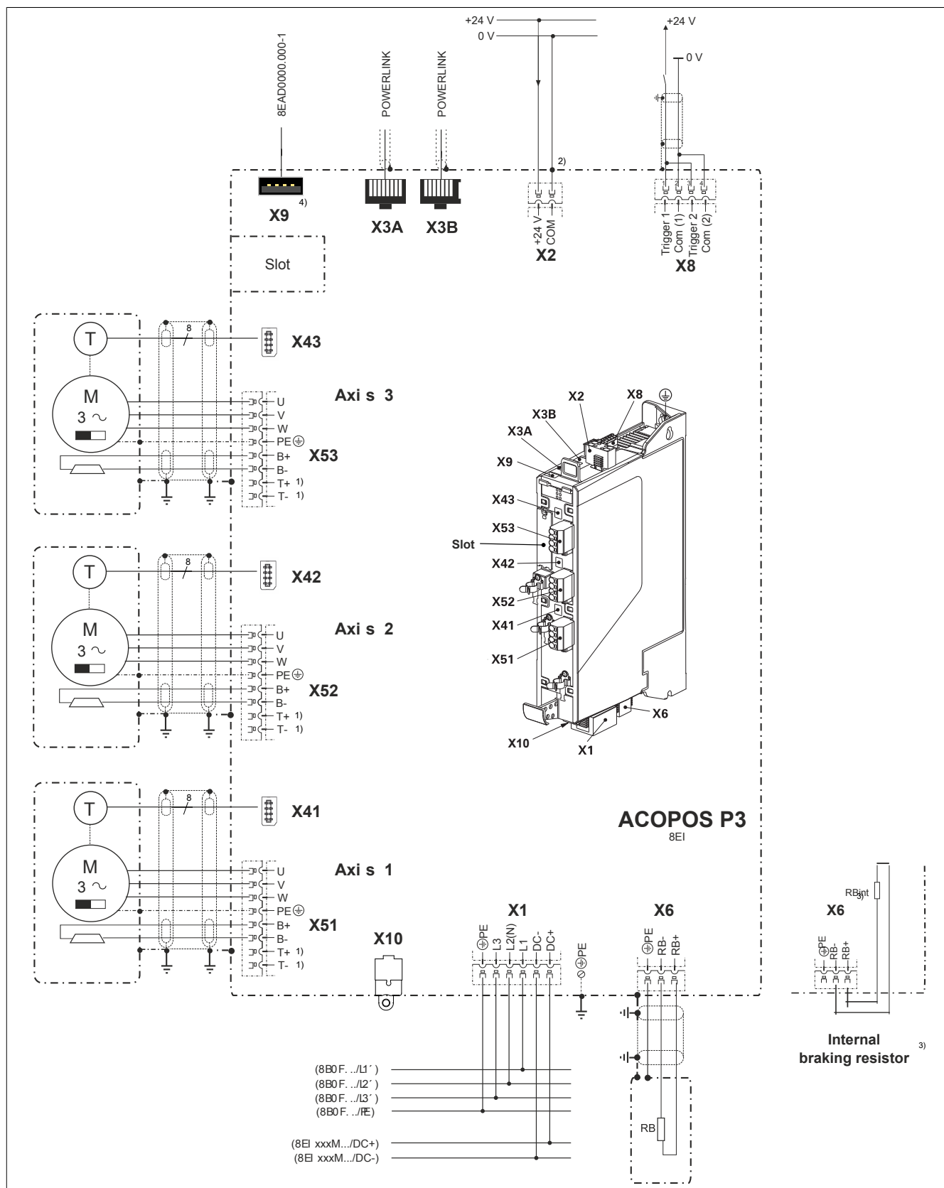
Figure 4: Mains input voltage - 1x 110 to 230 VAC / 3x 200 to 230 VAC
