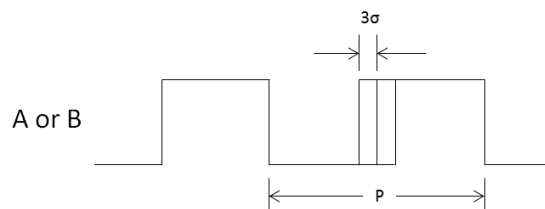
Figure 28: ABZ Jitter
