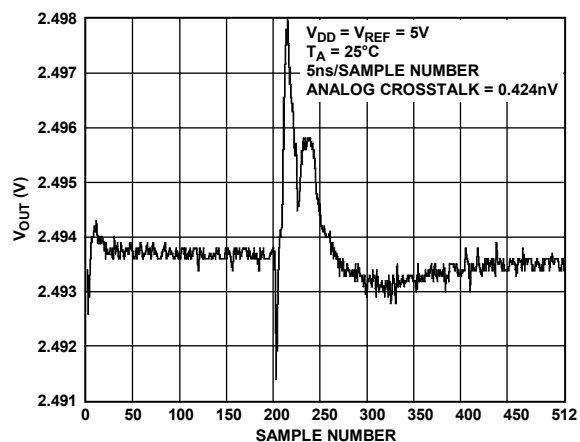
Figure 45. Analog Crosstalk, External Reference
