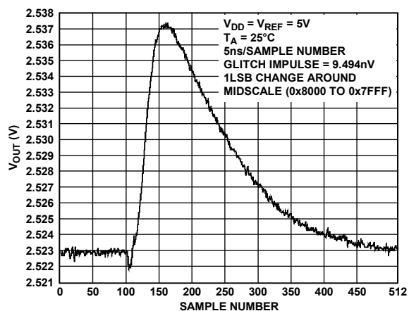
Figure 44. Digital-to-Analog Glitch Impulse (Negative)
