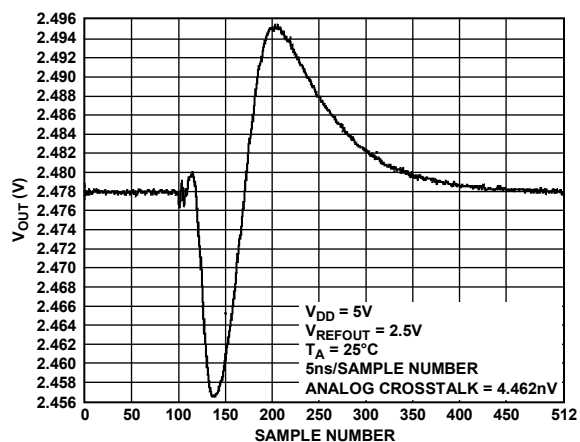
Figure 46. Analog Crosstalk, Internal Reference
