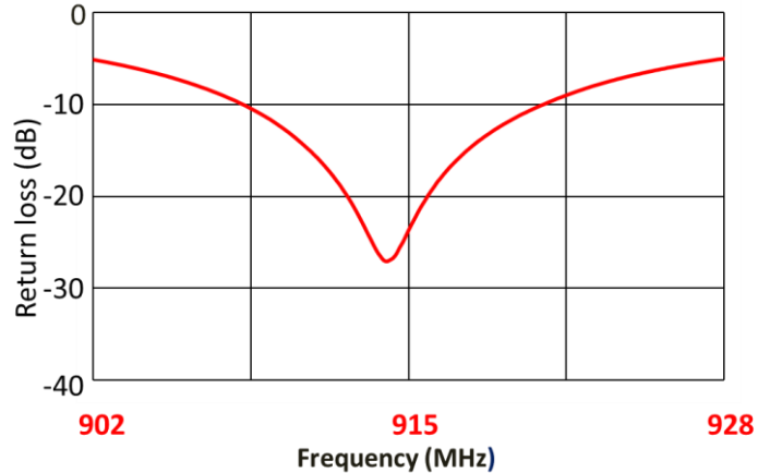
Return Loss
