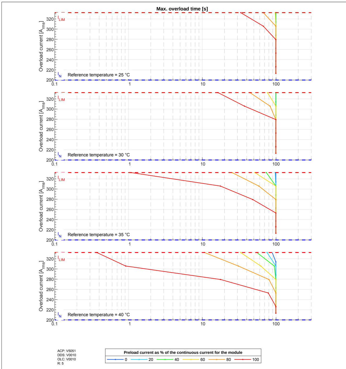
Figure 1: 8BVI2000HWSx.000-x - Overload characteristics, overload response - WARNING
