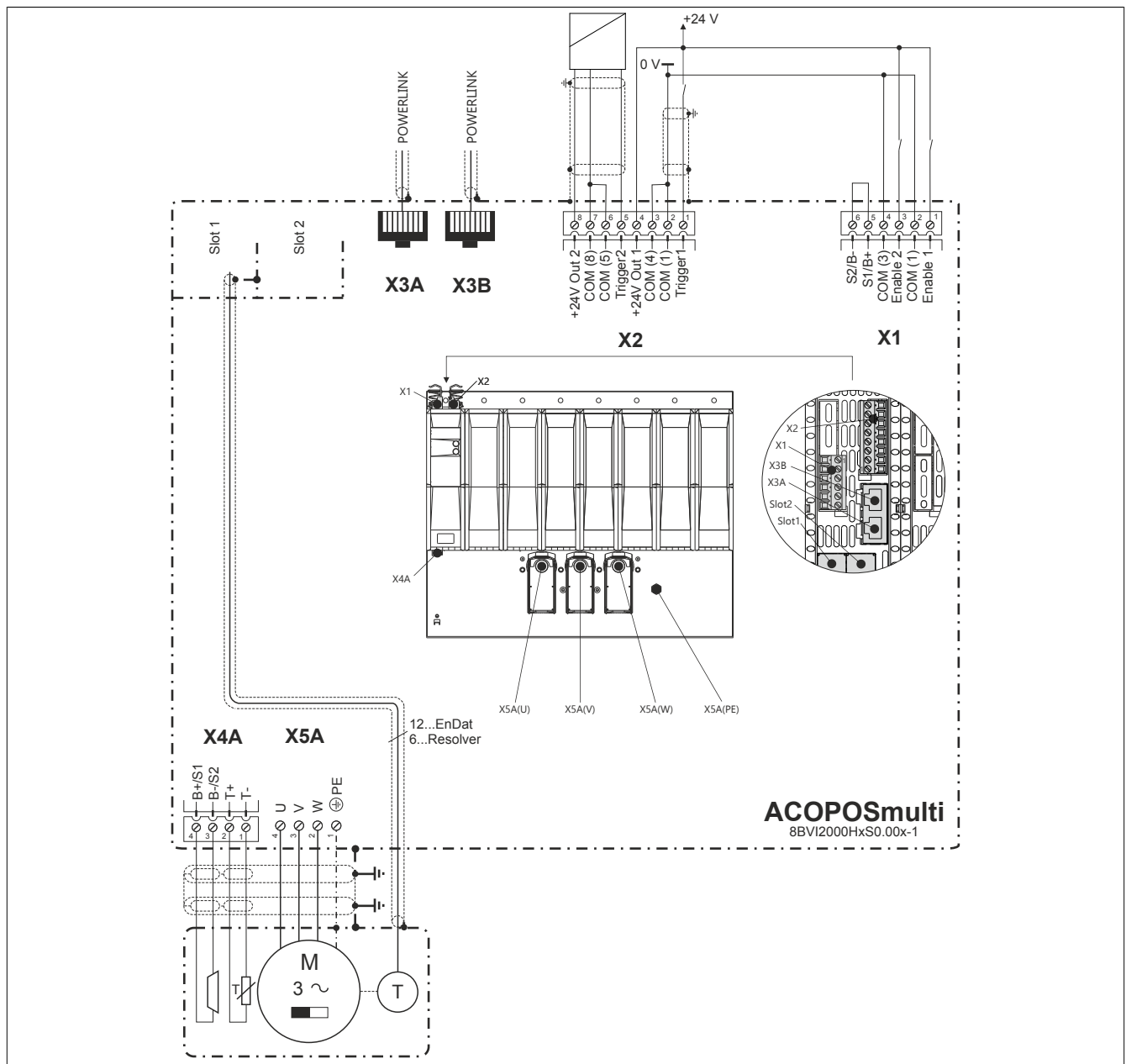
Figure 5: 8BVI2000HxS0.000-1 - Pinout overview
