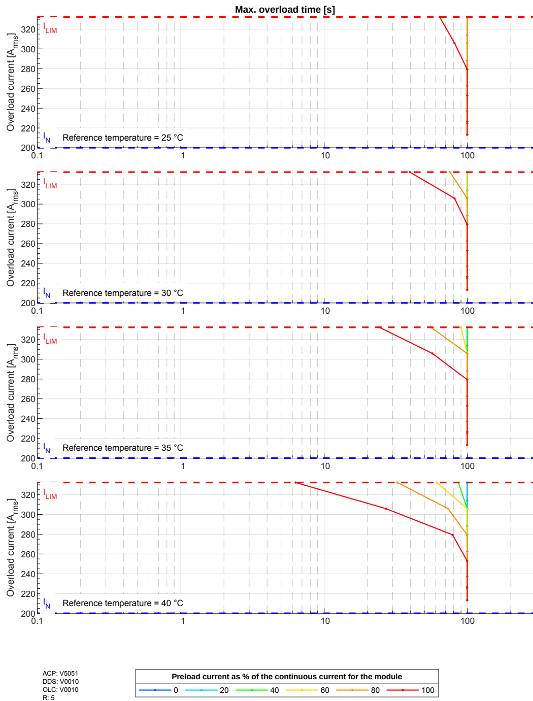
Figure 2: 8BVI2000HWSx.000-x - Overload characteristics, overload response - ERROR+STOP
