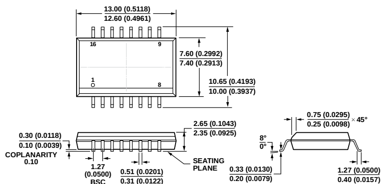
Dimensions shown in millimeters and (inches)
