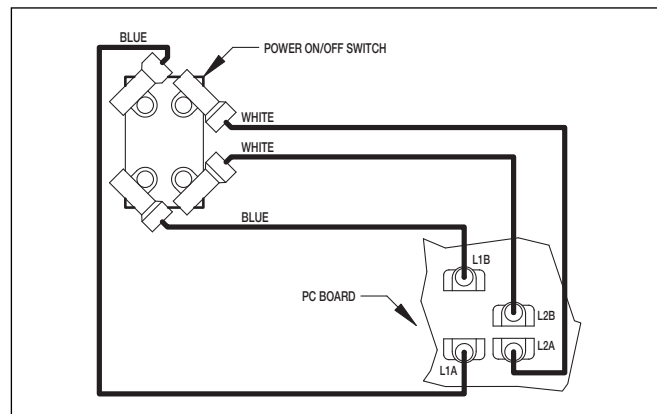
FIGURE 3 – CONNECTION DIAGRAM
