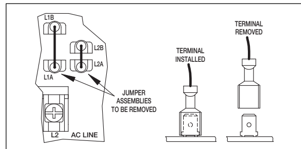
FIGURE 2 – TYPICAL LAYOUT OF JUMPER ASSEMBLIES
