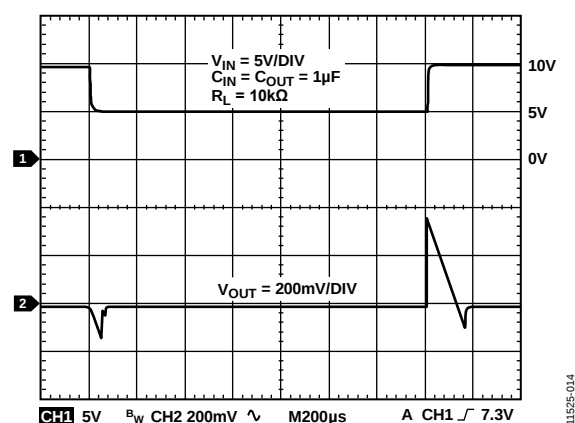
Figure 20. Line Transient Response (see Figure 25)
