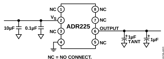
Figure 24. Basic Voltage Reference Connections
