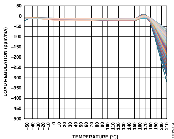
Figure 13. Load Regulation vs. Temperature ( I_{LOAD} = 0 \text{ mA to } 10 \text{ mA} ), FLATPACK Package
