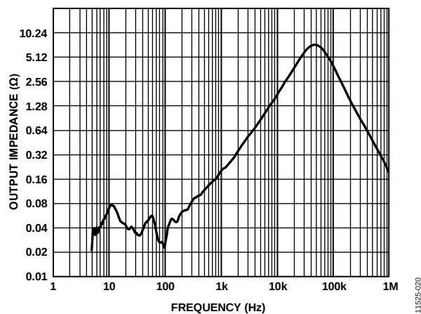
Figure 23. Output Impedance ( Z_{OUT} ) vs. Frequency, C_{IN} = C_{OUT} = 1 \mu F
