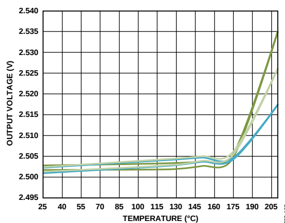
Figure 19. Thermal Hysteresis, I_{LOAD} = 0 mA, FLATPACK Package
