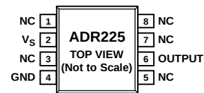
Figure 1. Pin Configuration for SOIC and FLATPACK Packages
