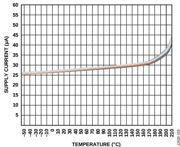
Figure 12. Supply Current ( I_{SV} ) vs. Temperature, FLATPACK Package
