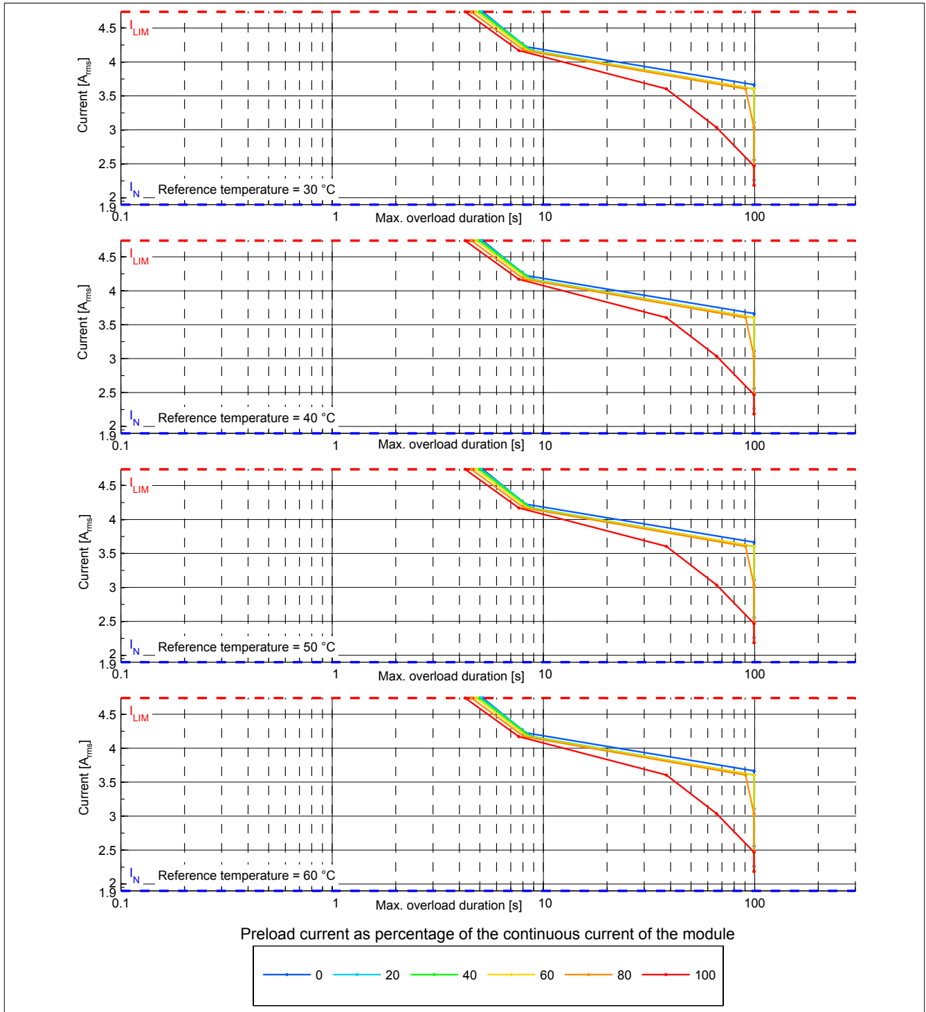
Figure 1: 8BVI0014HCDx.000-x - Overload characteristics, overload response - WARNING
