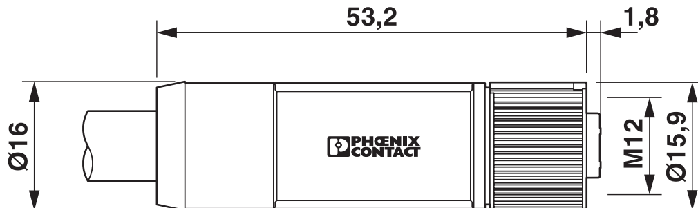
Dimensional drawing
