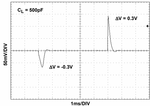
FIGURE 48. LINE TRANSIENT RESPONSE
