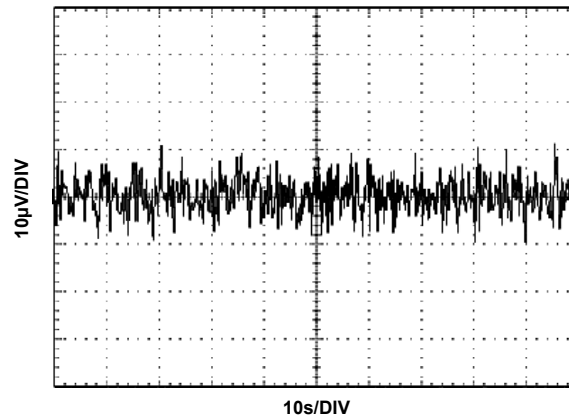
FIGURE 83. V_{OUT} NOISE
