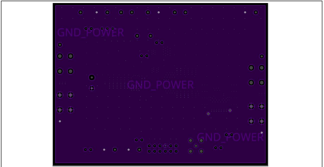
Figure 4 Inner layer 1
