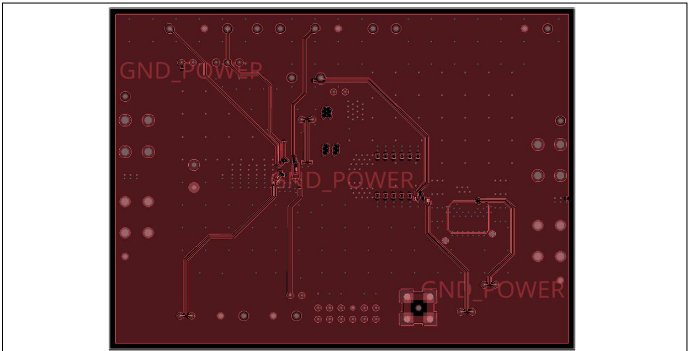
Figure 5 Inner layer 2
