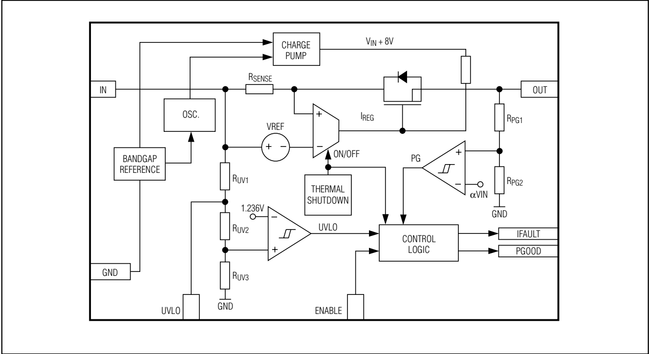
Functional Diagram
