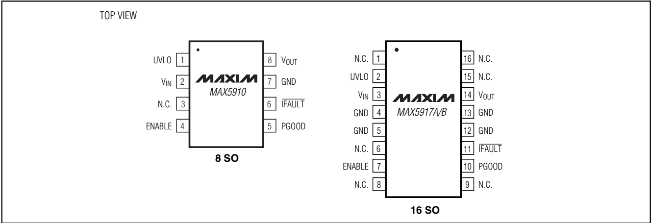
Pin Configurations
