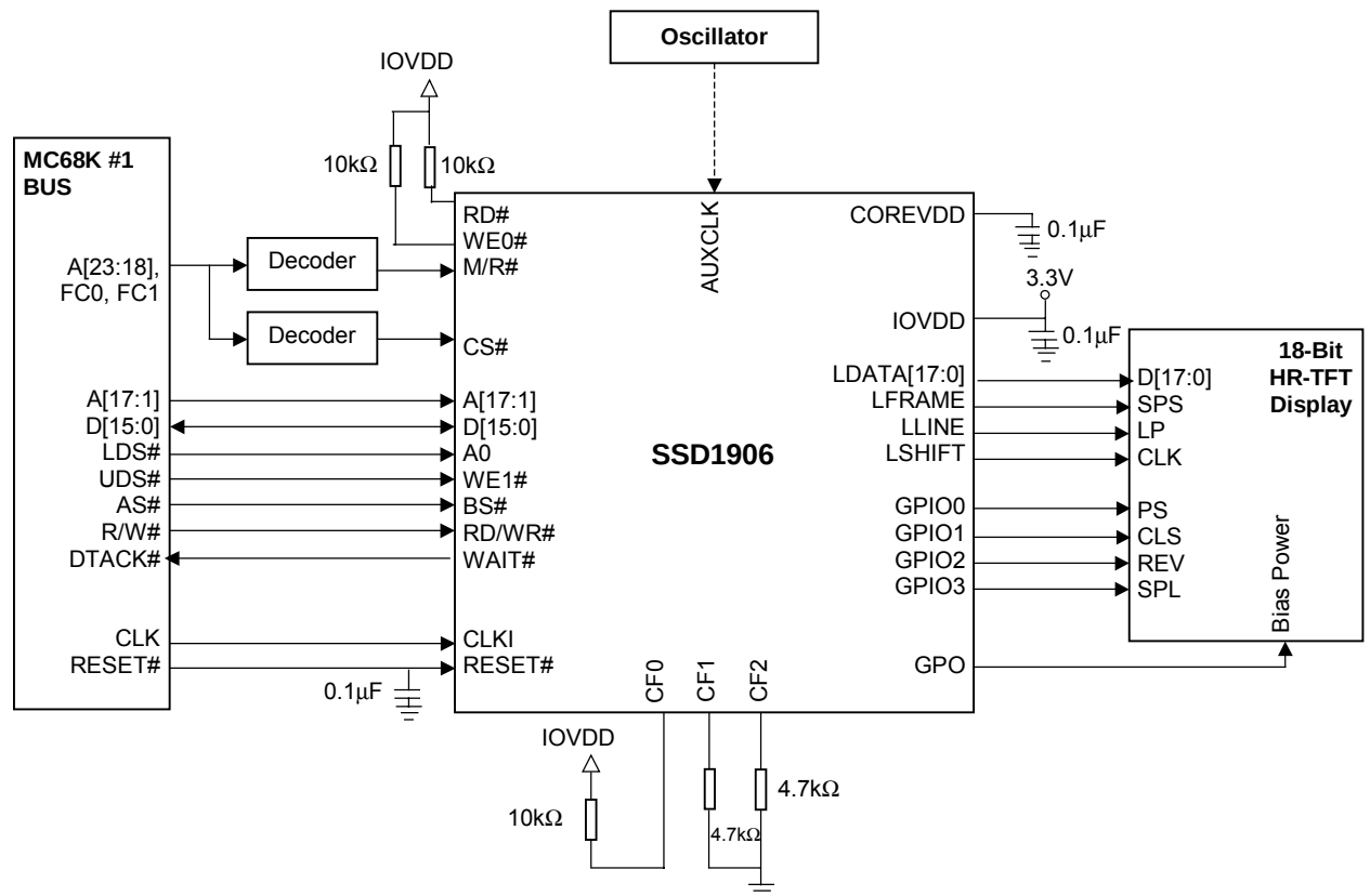
Figure 21-3 : Typical System Diagram (MC68K # 1, Motorola 16-Bit 68000)
