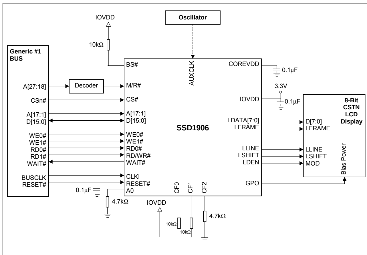
Figure 21-1: Typical System Diagram (Generic #1 Bus)
