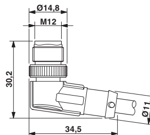
Dimensioned drawing
