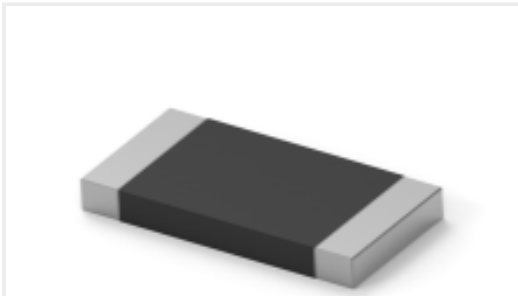
TE Part #2176422-6 TLRP 2512 3.0W R020 1% 75PPM 4K RL
