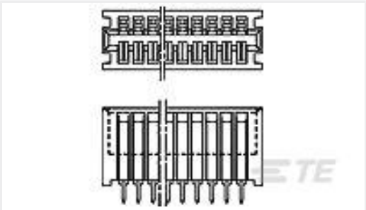
TE Part #166086-6 SINGLE LOADED/OPEN ENDS
